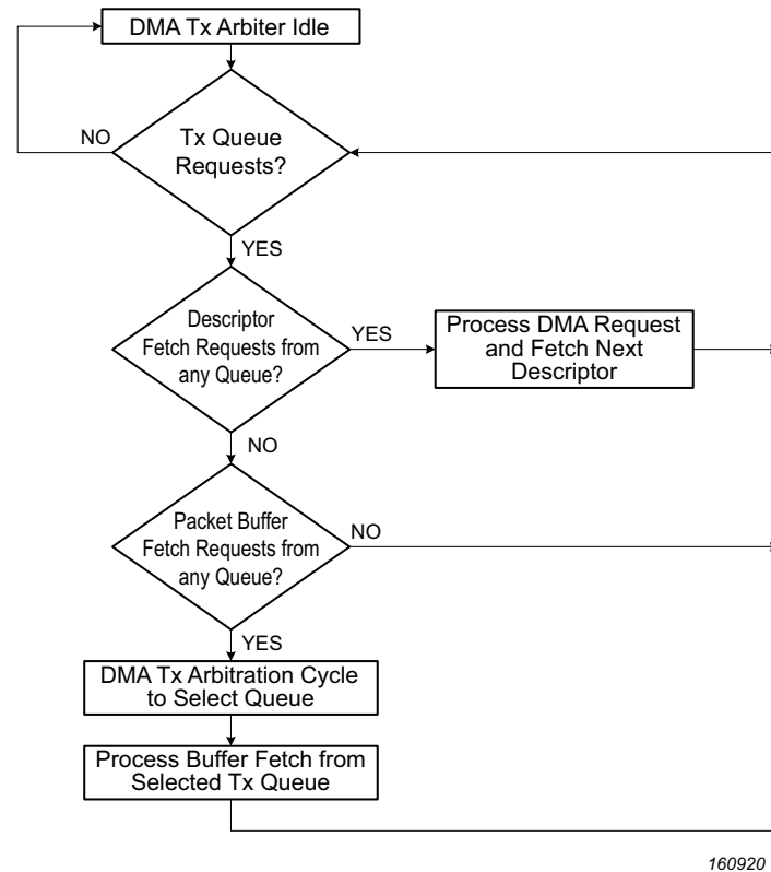
Fig 152. DMA transmit channel arbitration process
