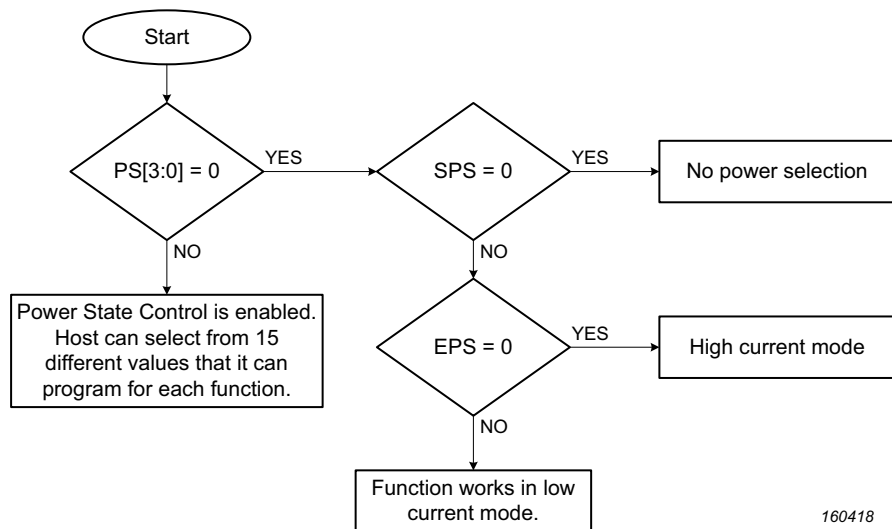
Fig 97. Flowchart for detect and program power requirements of functions
