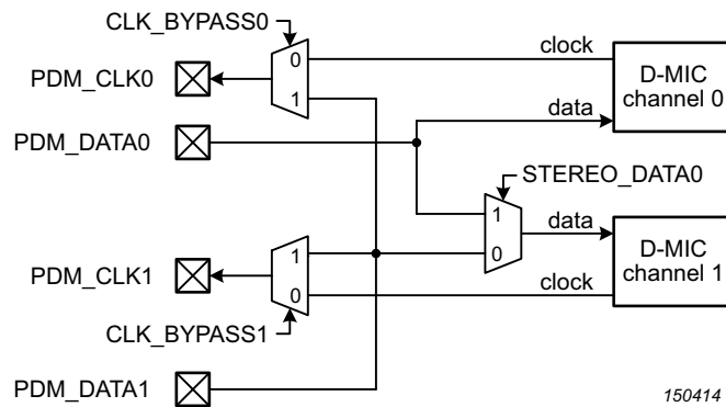
Fig 76. DMIC subsystem pin multiplexing
