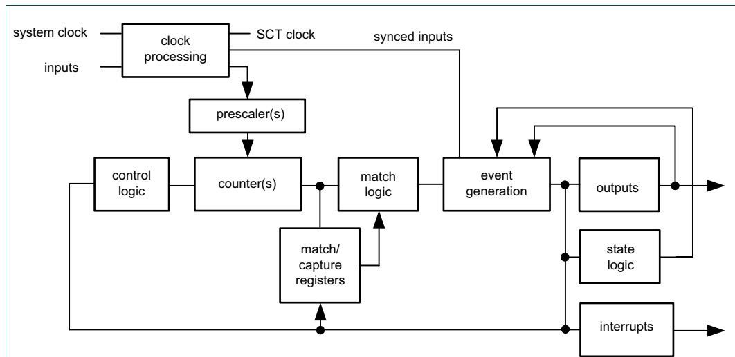
Fig 30. SCTimer/PWM block diagram
