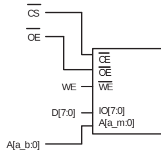
Fig 116. 8 bit bank external memory interface (bits MW = 00)
