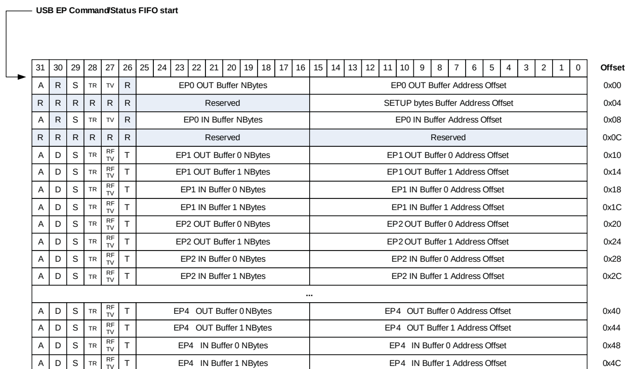
Fig 163. Endpoint command/status list (see also Table 822 )
