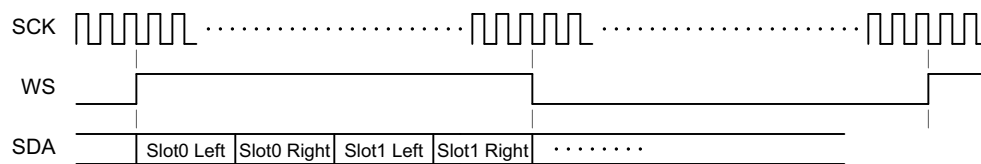
Fig 68. TDM in classic I 2 S mode
