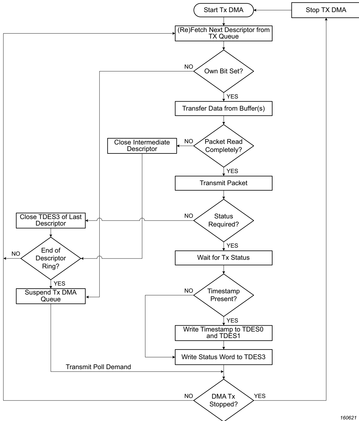
Fig 150. Transmit DMA operation in default mode
