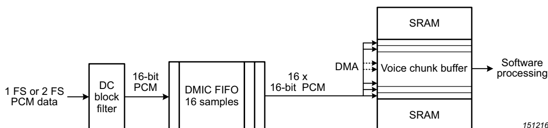
Fig 89. DMIC FIFO and DMA
