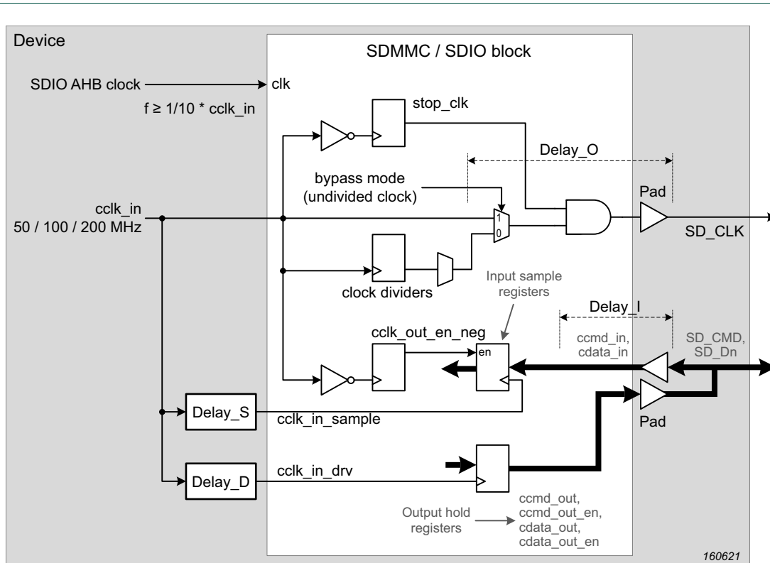
Fig 104. Different clocks and delays
