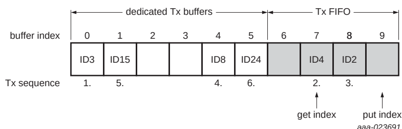
Fig 141. Example of mixed configuration dedicated Tx buffers / Tx FIFO
