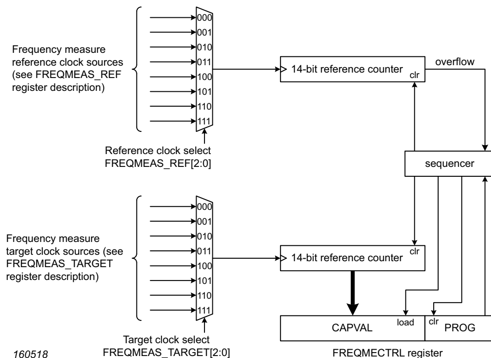
Fig 12. Frequency measure block diagram
