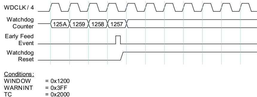
Fig 45. Early watchdog feed with windowed mode enabled
