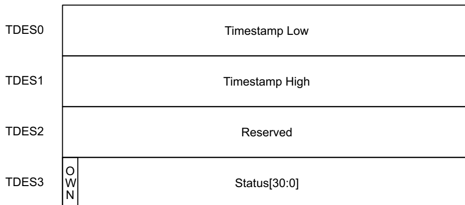
Fig 157. Transmitter descriptor write-back Format
