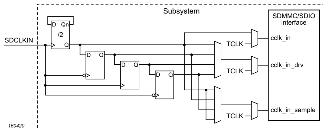
Fig 106. Clock phase-shift technique
