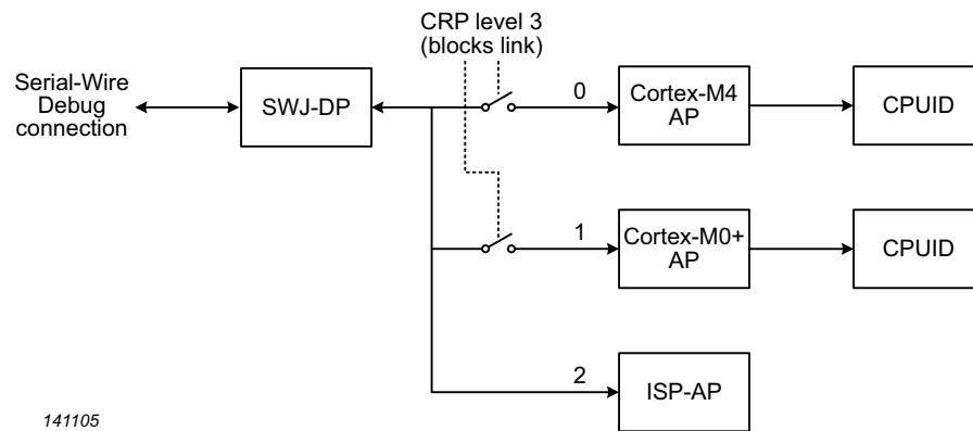
Fig 182. Serial Wire Debug internal connections
