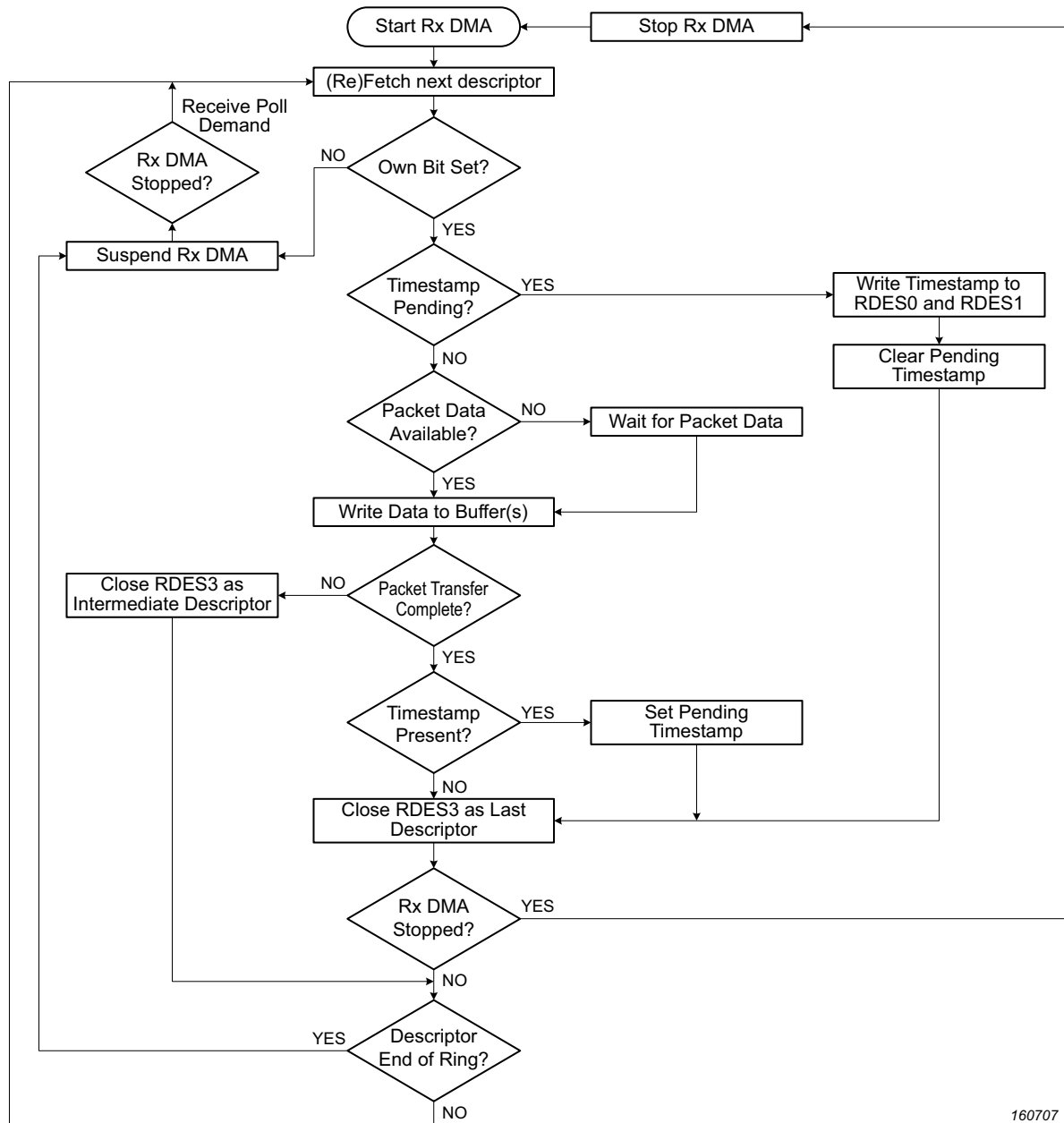
Fig 153. Receive DMA operation
