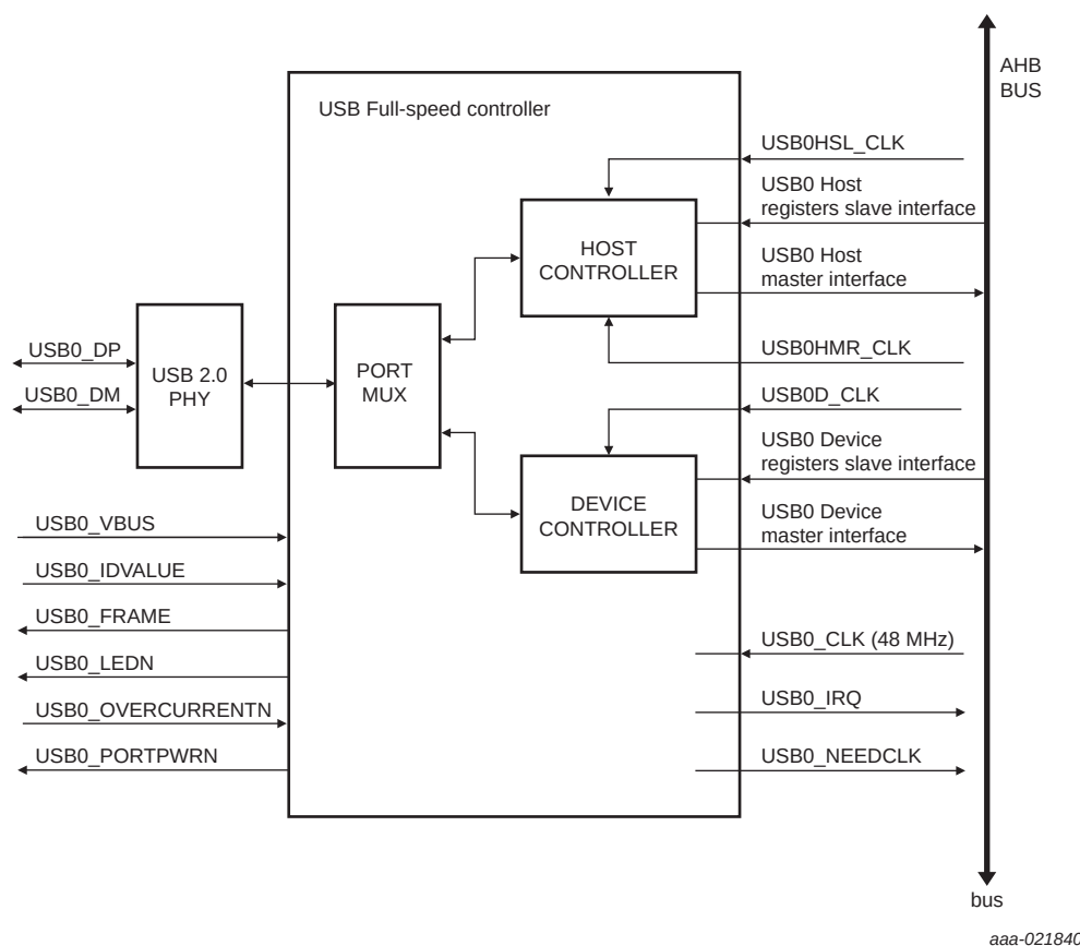
Fig 161. USB Full-speed host/device controller block diagram
