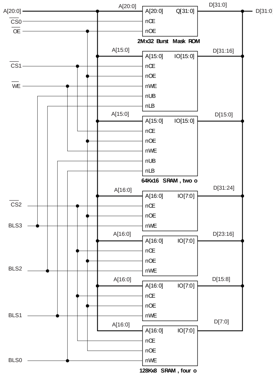
Fig 117. Typical memory configuration diagram
