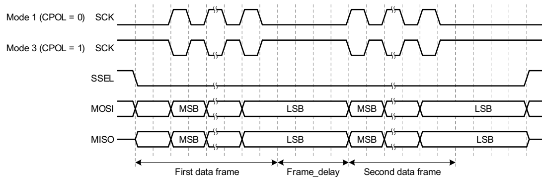
Fig 59. Frame_delay
