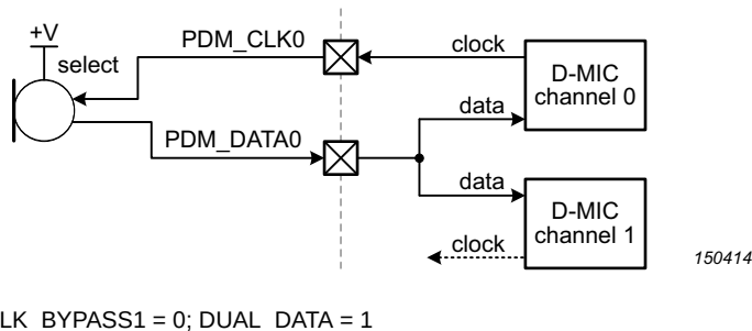
Fig 79. Typical connection to a stereo microphone
