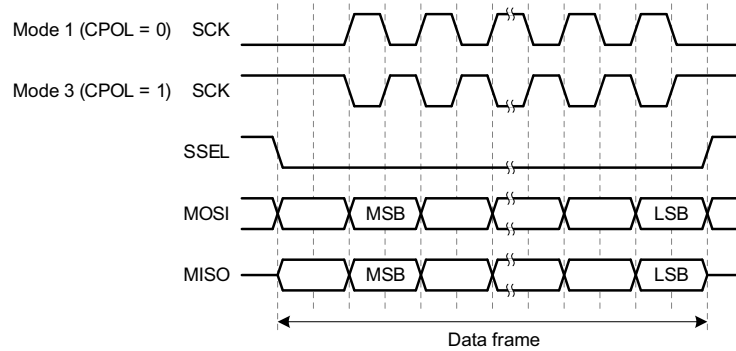
Fig 57. Basic SPI operating modes
