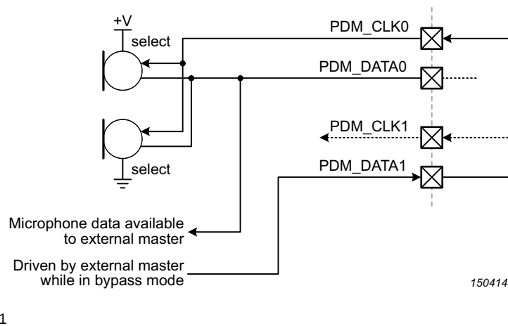
Fig 80. Bypass mode with an external device taking over microphone access
