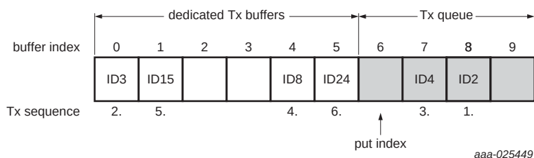
Fig 142. Example of mixed configuration dedicated Tx buffers / Tx queue
