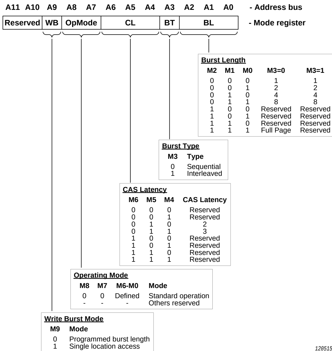
Fig 113. SDRAM mode register
