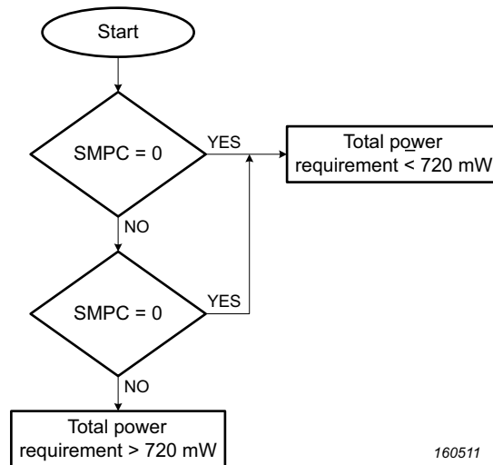
Fig 95. Flowchart for card power requirements
