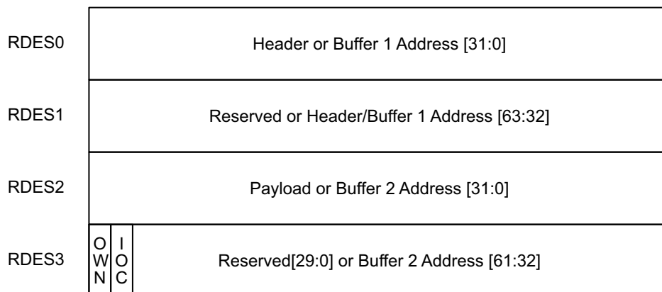
Fig 158. Receive normal descriptor (read format)
