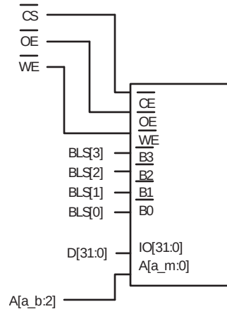
Fig 114. 32 bit bank external memory interfaces (bits MW = 10)
