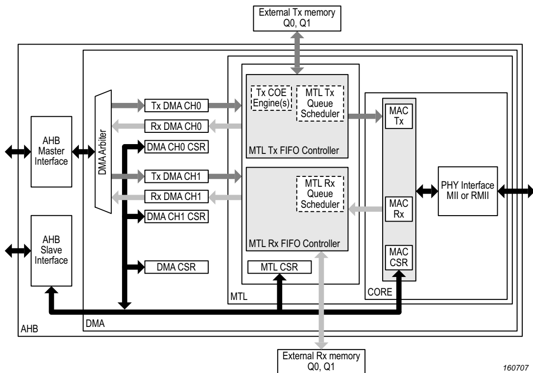
Fig 145. Multiple channels and queues
