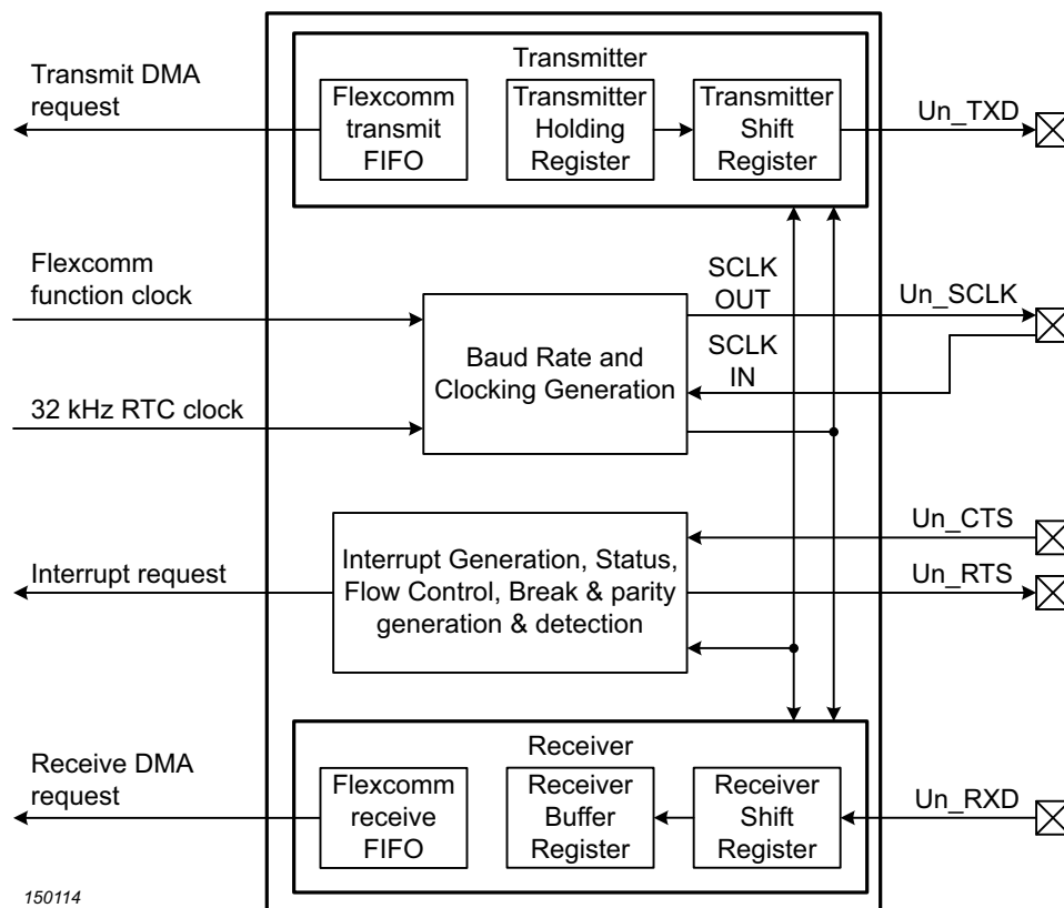
Fig 54. USART block diagram
