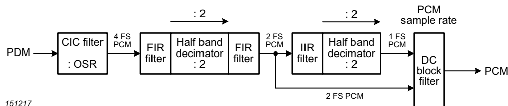
Fig 88. Principle structure of the PDM to PCM conversion
