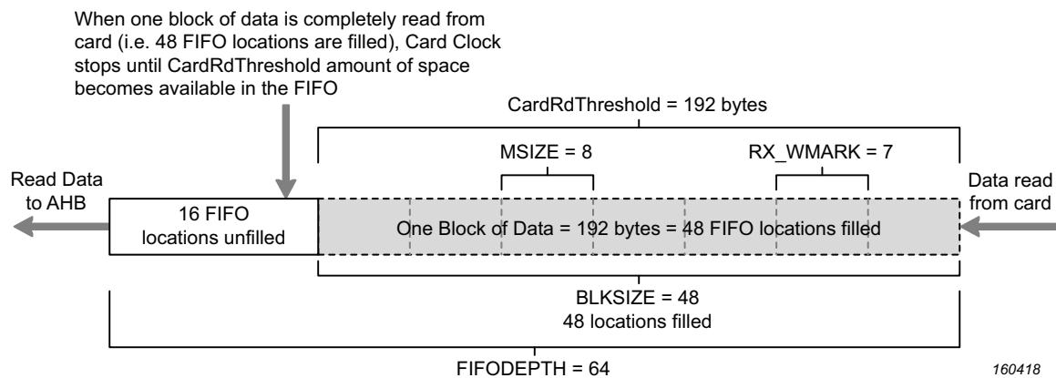
Fig 92. FIFO contents when BlkSize > \frac{1}{2} FifoDepth
