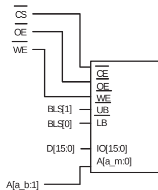
Fig 115. 16 bit bank external memory interfaces (bits MW = 01)
