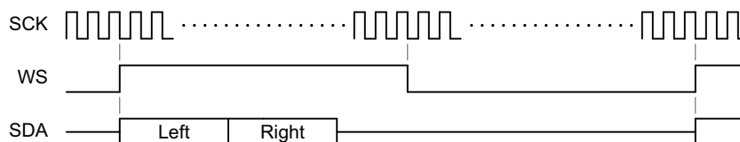
Fig 65. DSP mode with 50% WS
