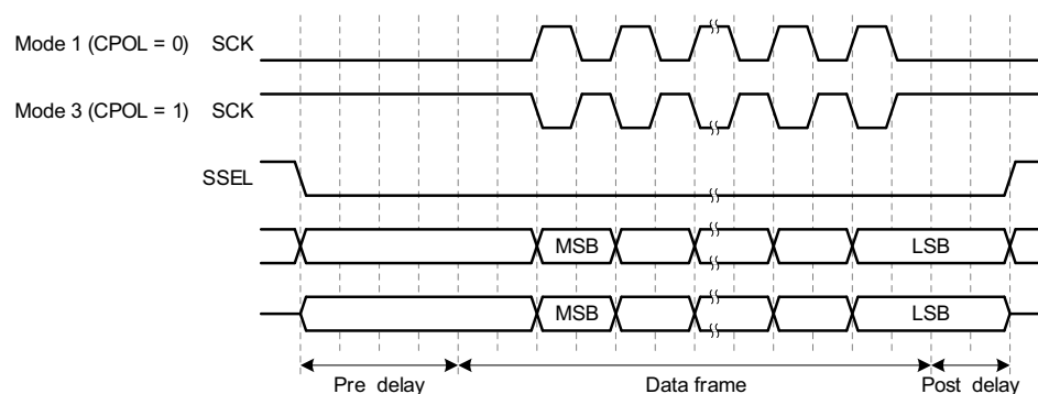
Fig 58. Pre_delay and Post_delay
