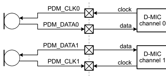
Fig 77. Typical connection to two independent microphones
