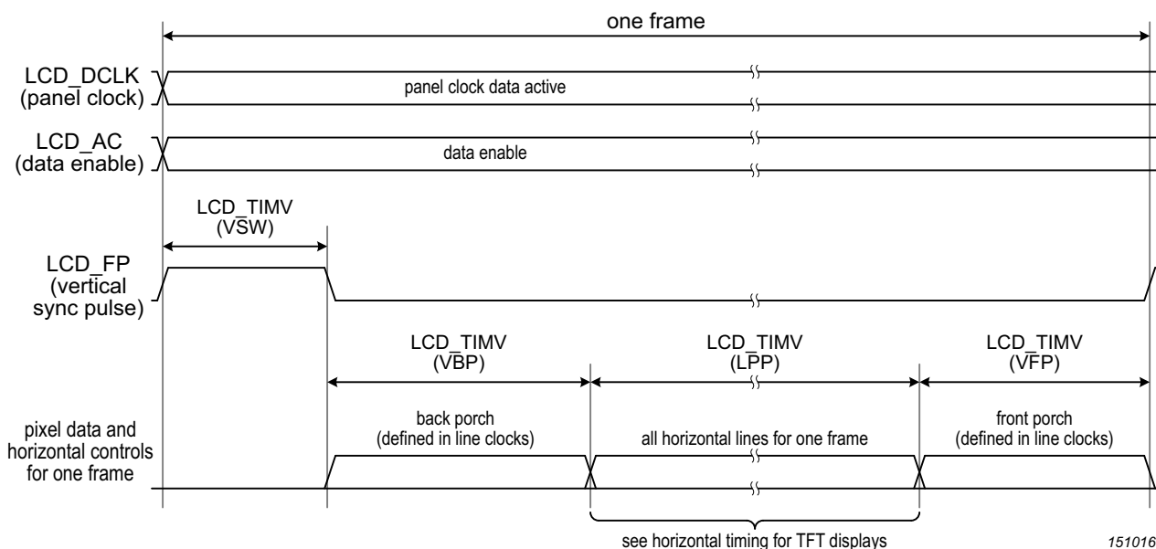
Fig 126. Vertical timing for TFT displays
