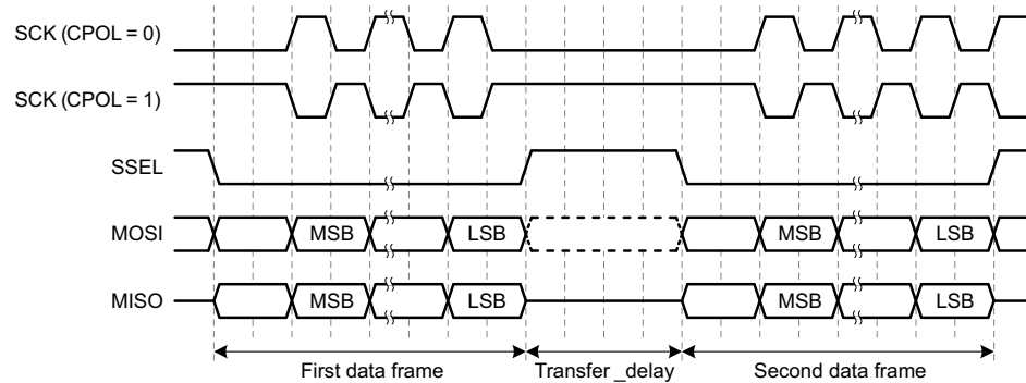
Fig 60. Transfer_delay
