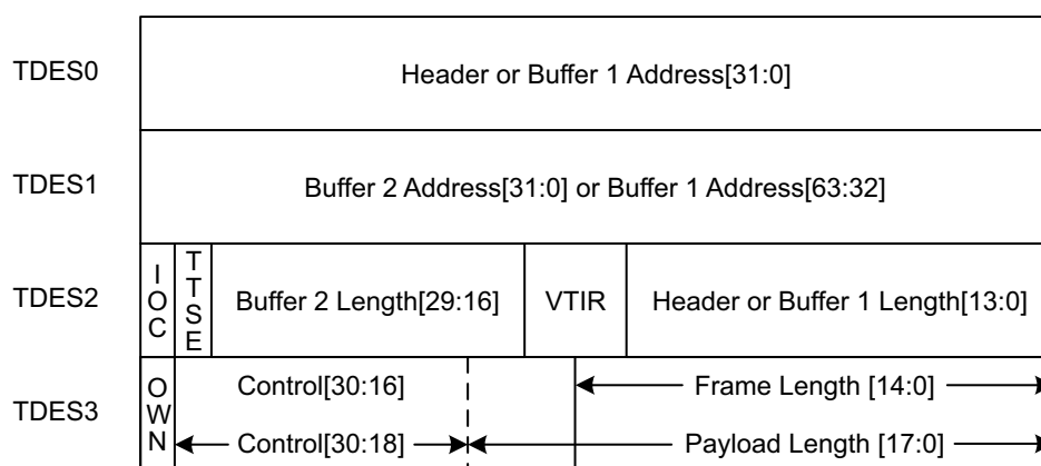
Fig 156. Transmitter descriptor read format
