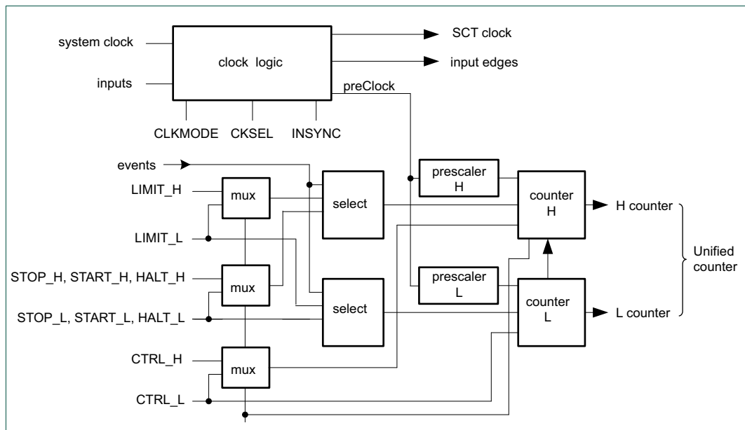
Fig 31. SCTimer/PWM counter and select logic
