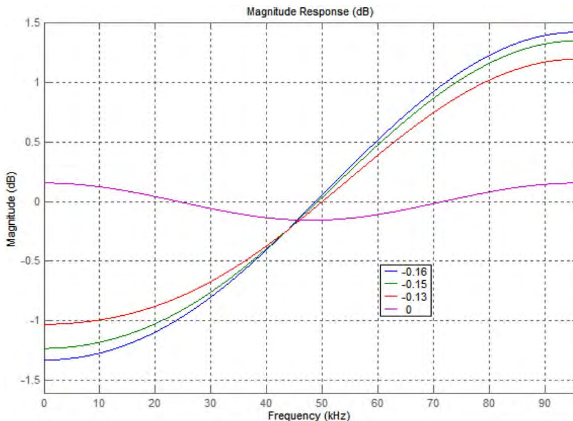
Fig 82. Pre-emphasis filter quantized response at 96 kHz
