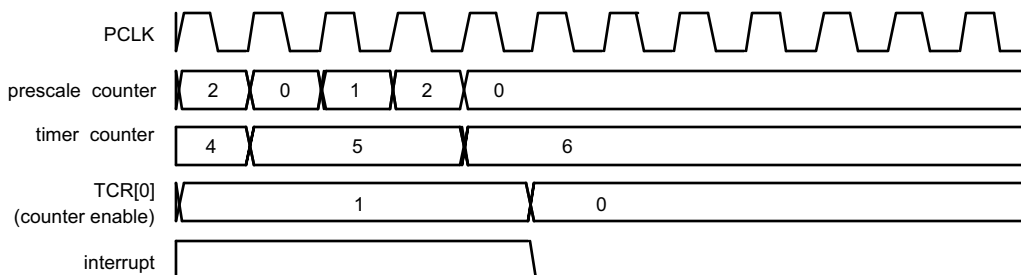
Fig 41. A timer cycle in which PR=2, MRx=6, and both interrupt and stop on match are enabled
