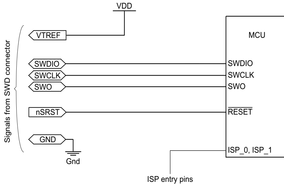
Fig 181. Connecting the SWD pins to a standard SWD connector
