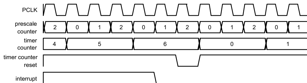
Fig 40. A timer cycle in which PR=2, MRx=6, and both interrupt and reset on match are enabled
