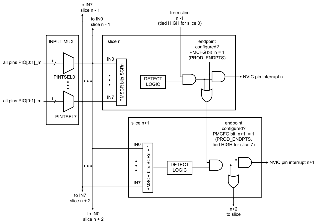
Fig 20. Pattern match engine connections
