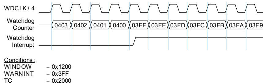
Fig 47. Watchdog warning interrupt
