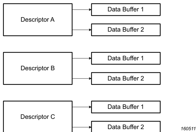
Fig 98. Dual buffer descriptor structure
