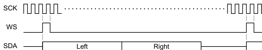
Fig 66. DSP mode with 1 SCK pulsed WS
