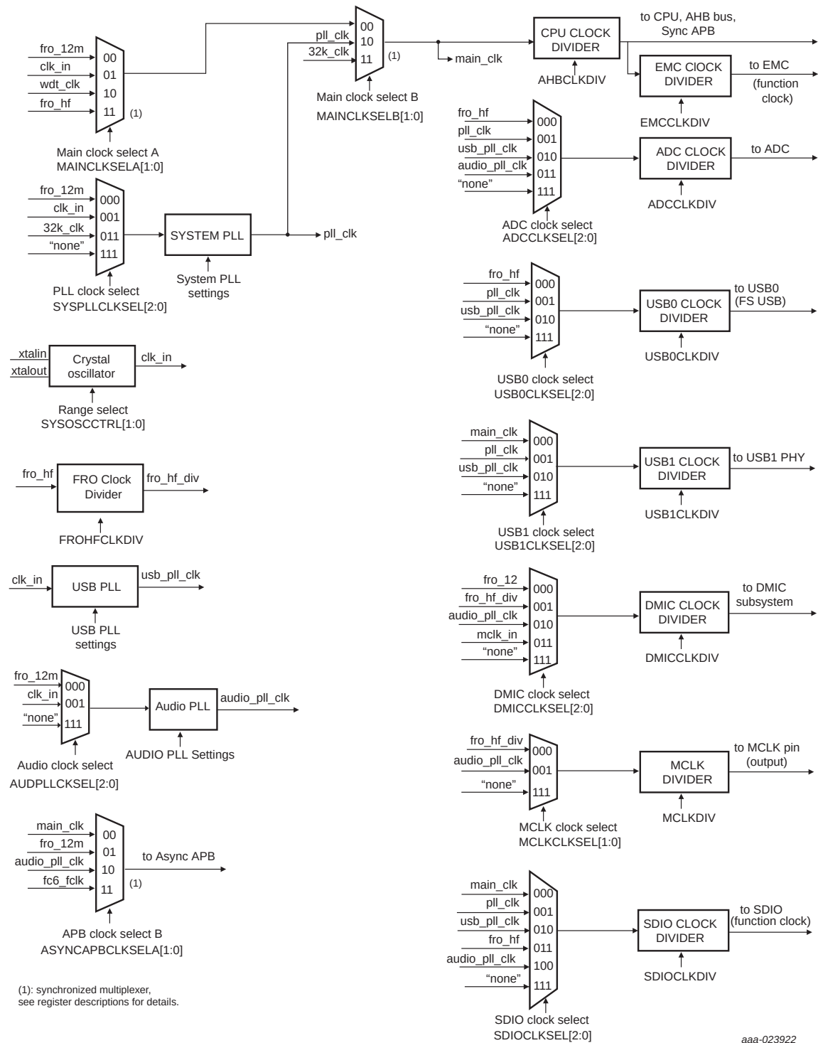
Fig 4. Clock generation
