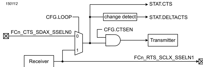
Fig 55. Hardware flow control using RTS and CTS
