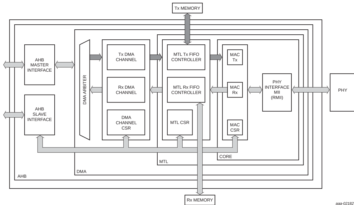
Fig 143. Ethernet block diagram
