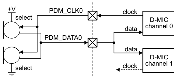
Fig 78. Typical connection to two microphones sharing a data line
