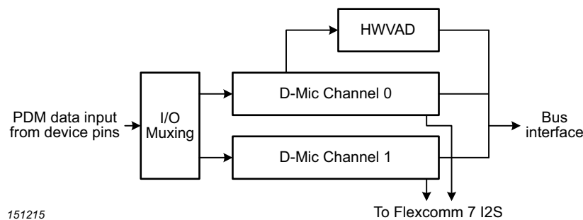
Fig 81. DMIC subsystem block diagram
