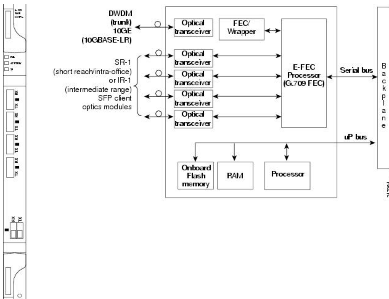
Figure 19: MXP 2.5G 10EX C Faceplate and Block Diagram
