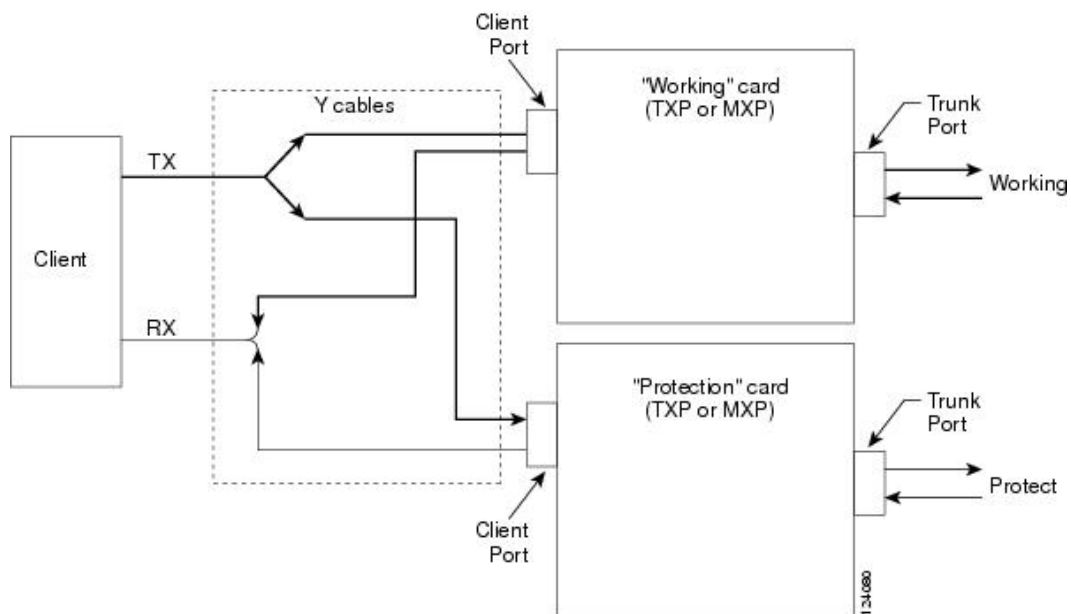
Figure 51: Y-Cable Protection
