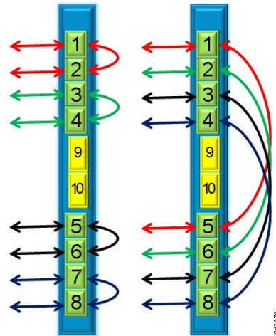
Figure 32: Low-Rate RGN Card Operating Mode Configuration
