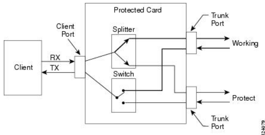
Figure 52: Splitter Protection
