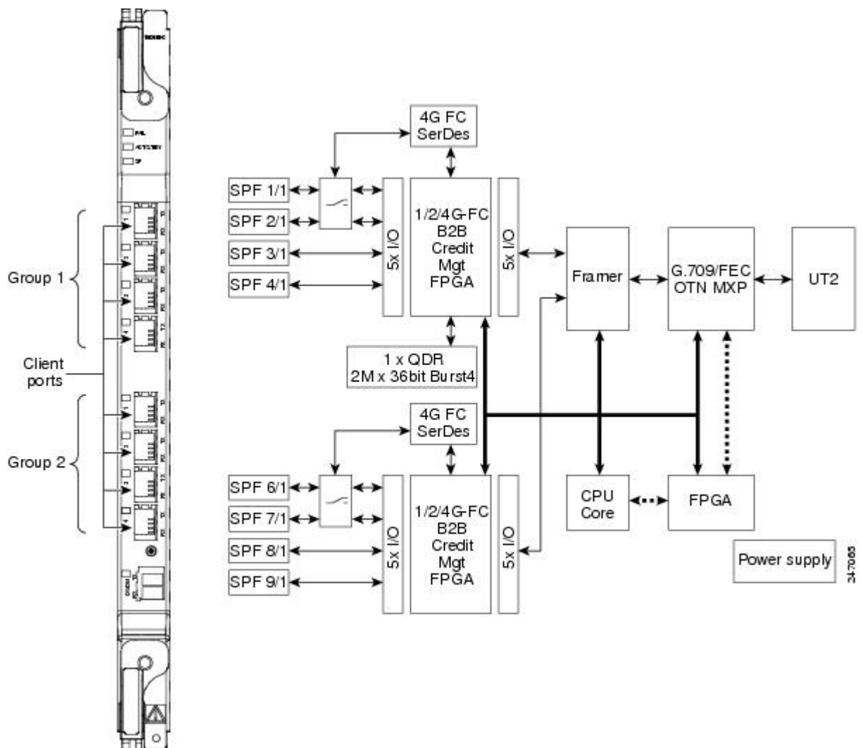
Figure 20: MXP_MR_10DMEX_C Faceplate and Block Diagram
