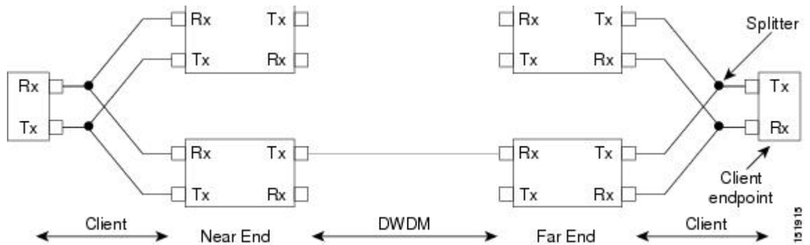
Figure 47: Y-Cable Protection
