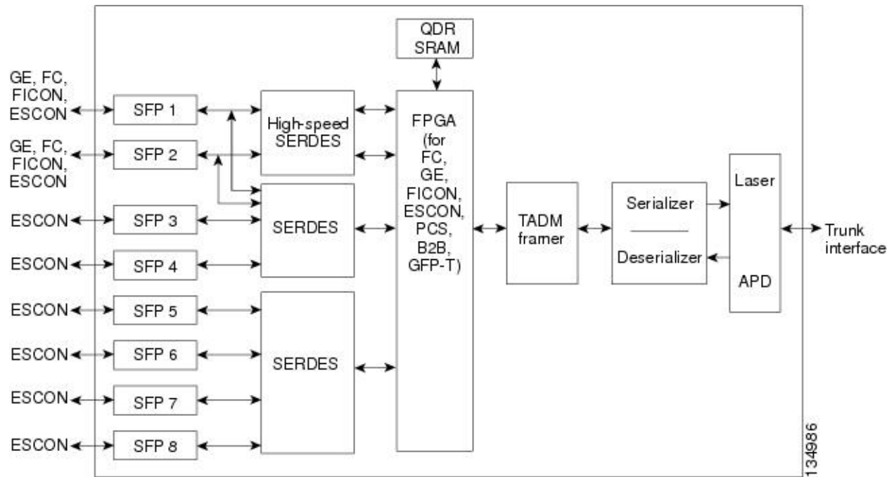
Figure 14: MXP_MR_2.5G and MXPP_MR_2.5G Block Diagram
