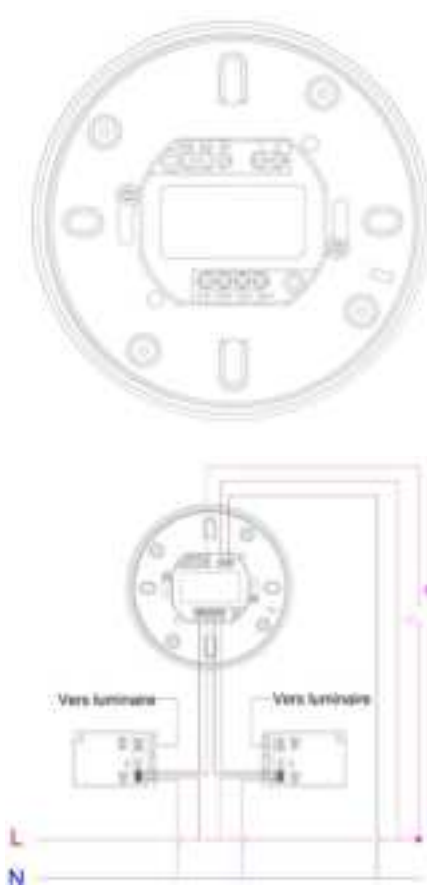
Version DALI
