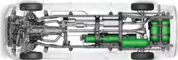
FOUR-TANK SYSTEM
