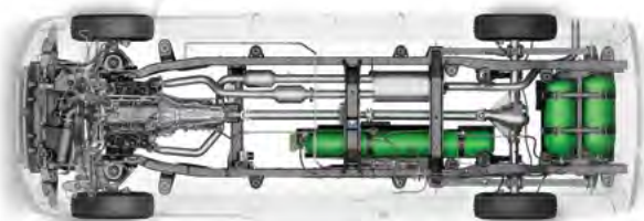
THREE-TANK SYSTEM
