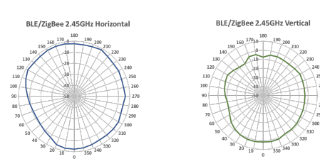
FAP-233G BLE/ZigBee antenna plots
