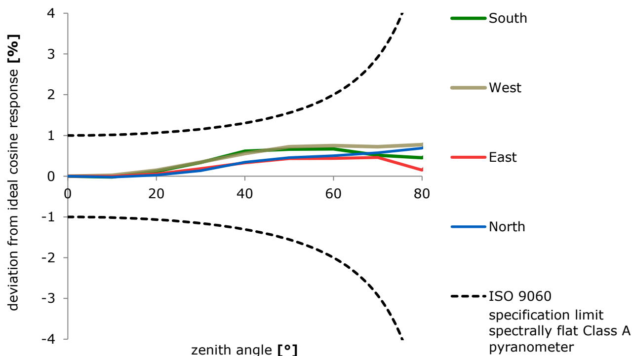
Figure 2.0.3 Directional response of an SR30 pyranometer of 4 azimuth angles, compared to spectrally flat Class A limits.
