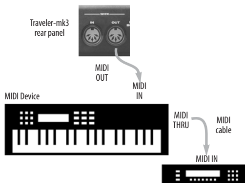
Figure 3-9: Connecting additional devices with MIDI THRU ports.
