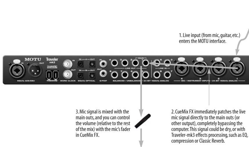
Figure 10-5: This diagram shows the signal flow when using CueMix FX no-latency monitoring. Notice that this method does not process the live input with plug-ins in your audio software. Instead, you can apply Traveler-mk3 effects, such as the reverb, EQ and/or compression.
