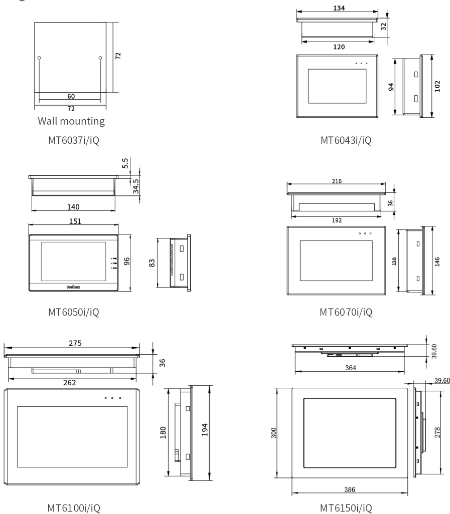
Diagram 1 Mounting size
