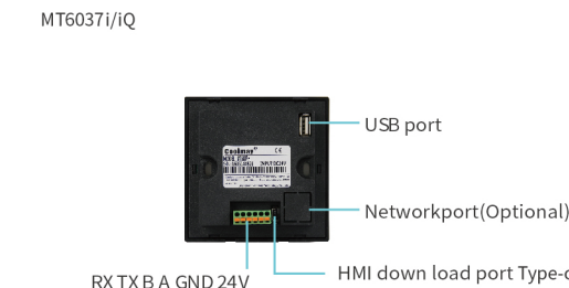
Diagram2 Product Structure
