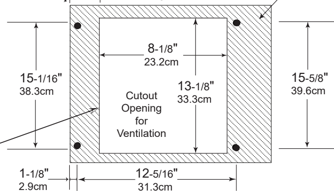
C12000 Preamplifier Bottom View in Custom Cabinet
