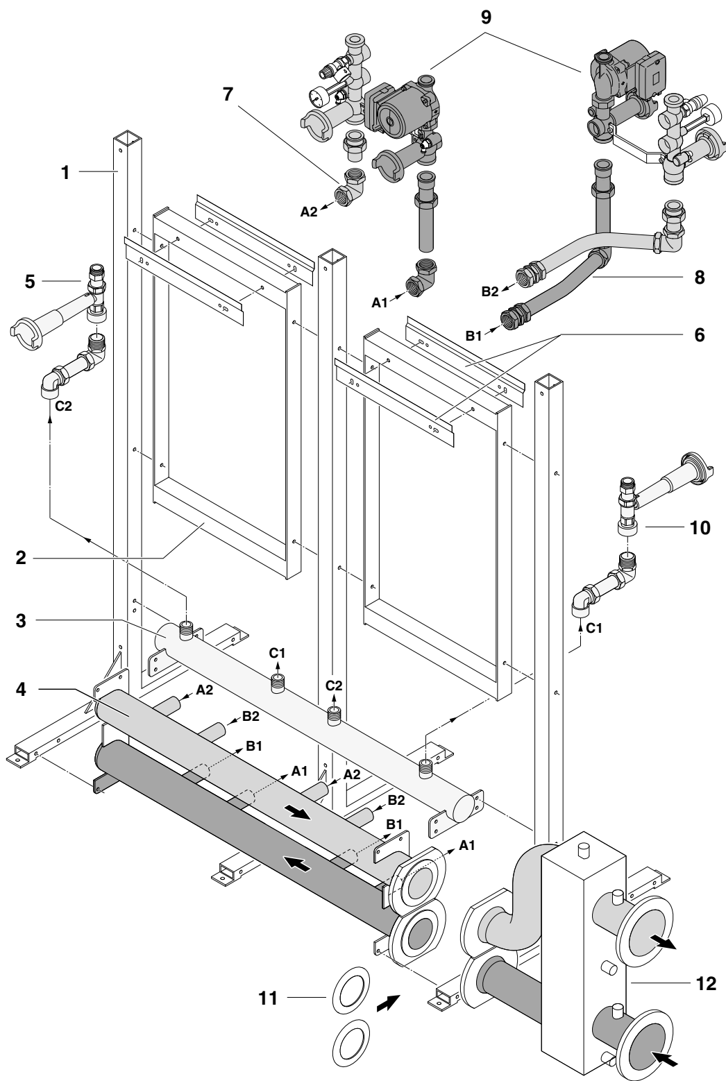
Fig. 1 Overview of Logamax plus GB162 cascade frame
