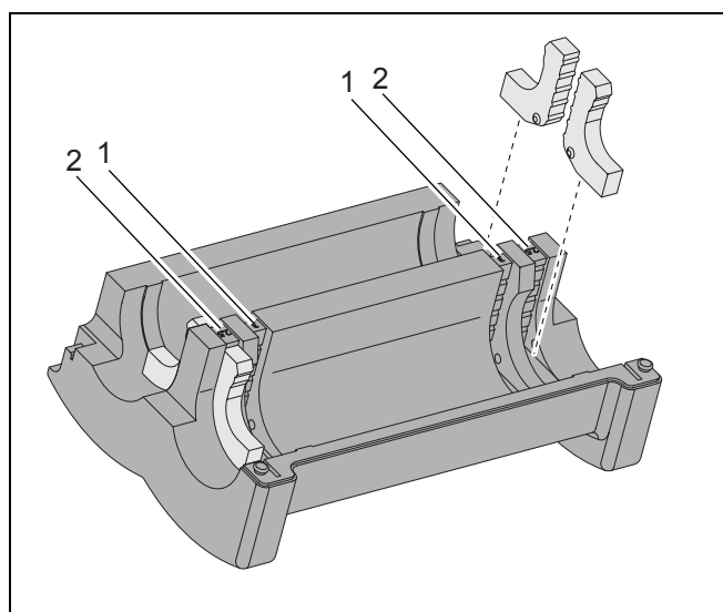
Fig. 10 Inner insulation
