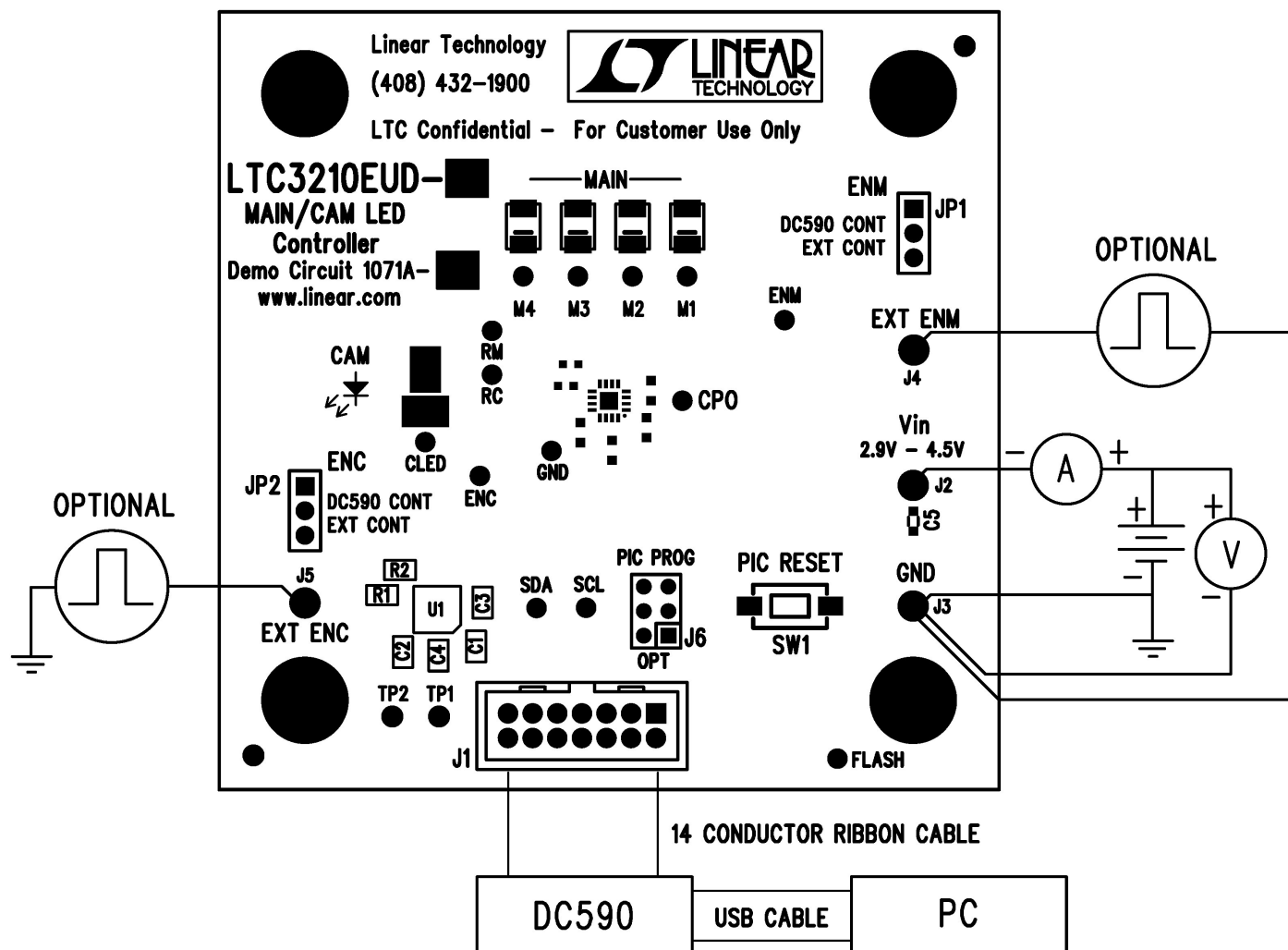
Figure 1. Proper Measurement Equipment Setup for DC1071A
