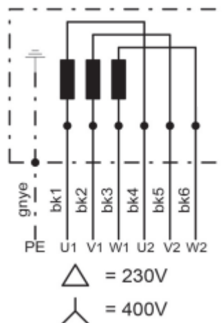
Wiring diagram Note:- 3 Phase fans are fitted with a flying lead.
