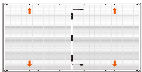
The outer four-hole bolt mounting, the beam perpendicular to the short frame
