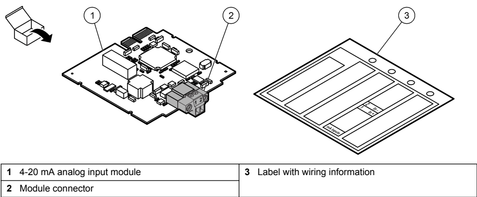
Figure 1 Product components
