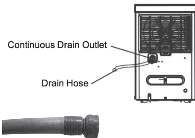
Continuous drain hose (ID \geq 5/16", not included) with a female threaded end (ID:M=1", not included.)
