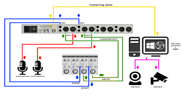
Wiring diagram for AIRERNCE mixer
