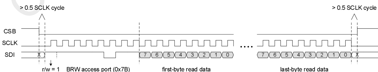
Figure 15. SPI (3-wire) BURST Read Register Timing
