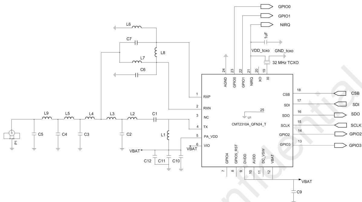
Figure 7. Application Schematic Diagram with TCXO
