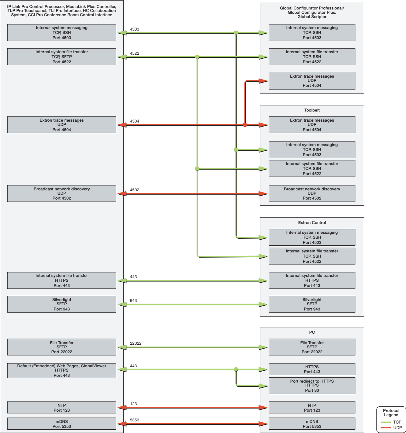
Figure 1. Interaction of Network Functions, Protocols, and Ports
