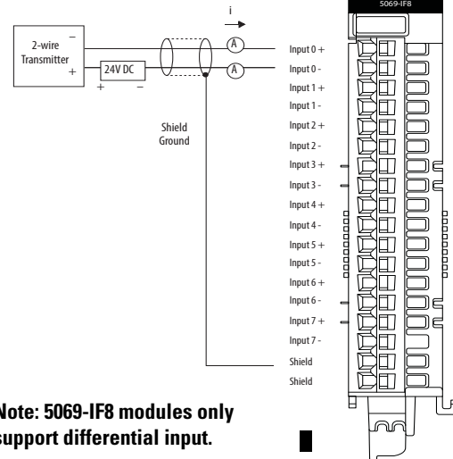
5069-IF8 Analog 8-channel Current/Voltage Input Module
