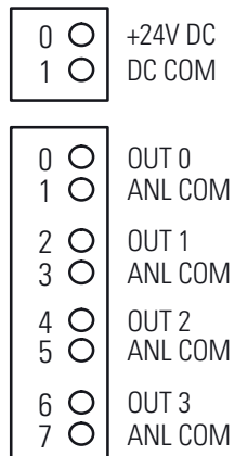
1746-N04I Analog Voltage Output Wiring
