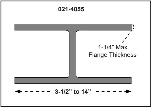
FIGURE 6 - INSTALLATION 021-4055
