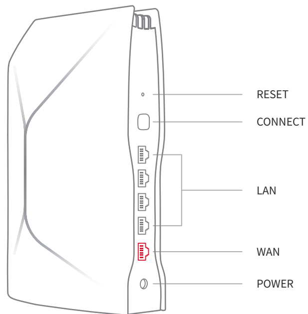
Port configuration
