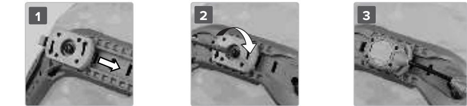
Figure 5 – MOLLE Mount
