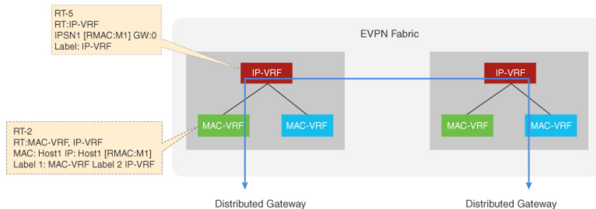
Figure 29: Symmetric IRB with MPLS on Distributed Gateways
