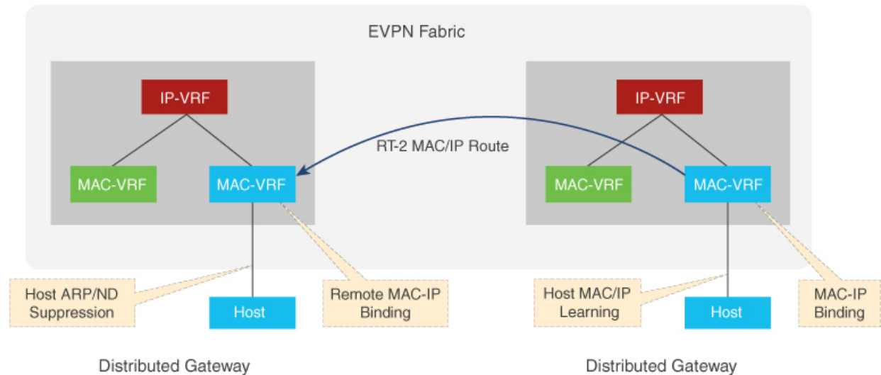
Figure 31: ARP and ND Flooding Suppression
