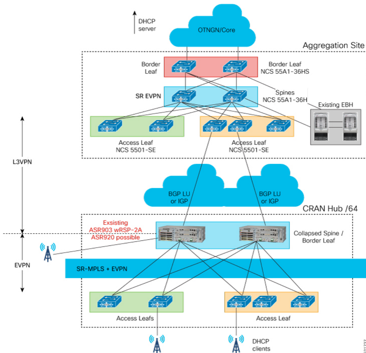
Figure 32: DHCP Relay Agent Network Topology
