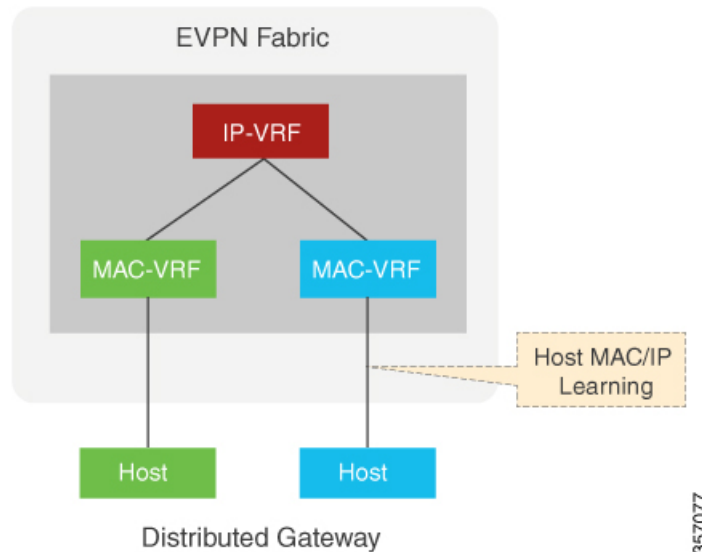
Figure 30: Host MAC-IP Binding on a Single-Homed DAG
