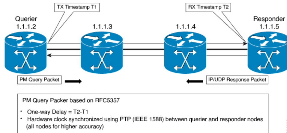
Figure 17: Performance Measurement for End-to-End Delay Measurement
