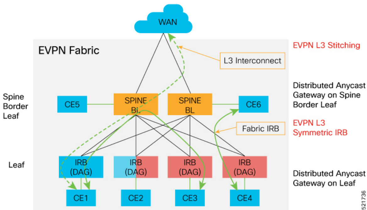
Figure 34: Collapsed Spine or Leaf or RR on a Single Node Network Topology
