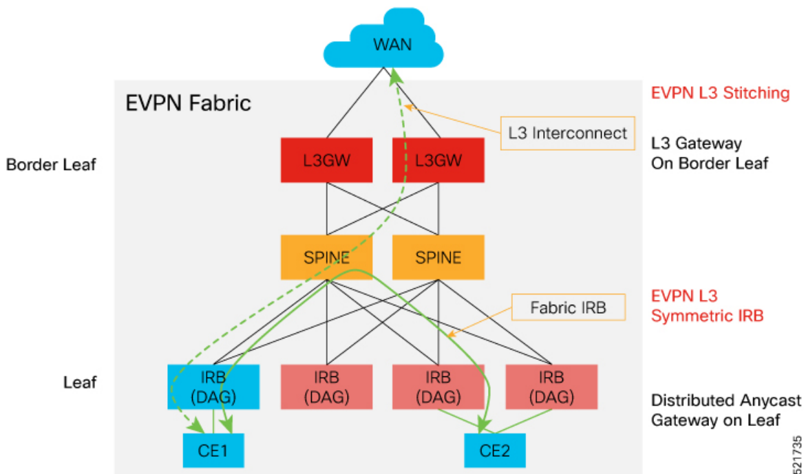
Figure 33: Single Homing DAGs with Symmetric IRB Network Topology
