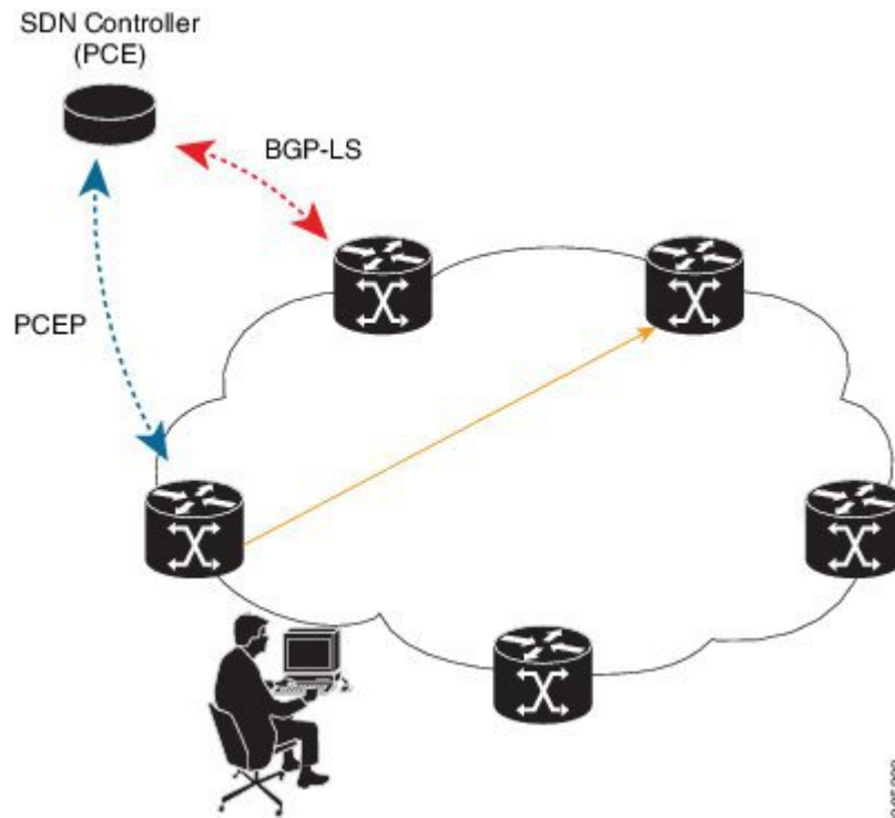
Figure 4: SDN Controller
