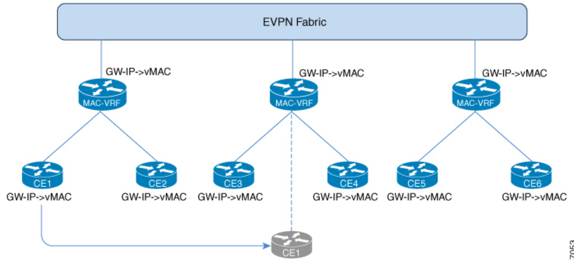
Figure 28: DAG with Bridge Domains
