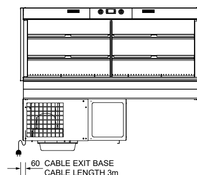
REAR ELEVATION
