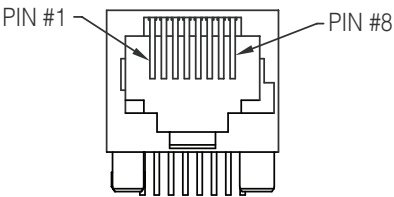
Figure 7. CAT 5 Connector Pin Details
