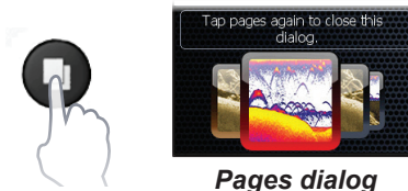
Pages dialog
