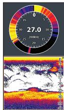
Split Flasher
