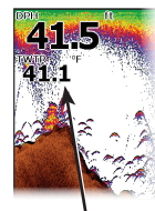
Overlay data
