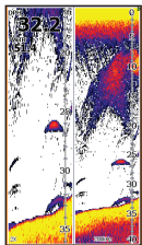
Split Zoom
