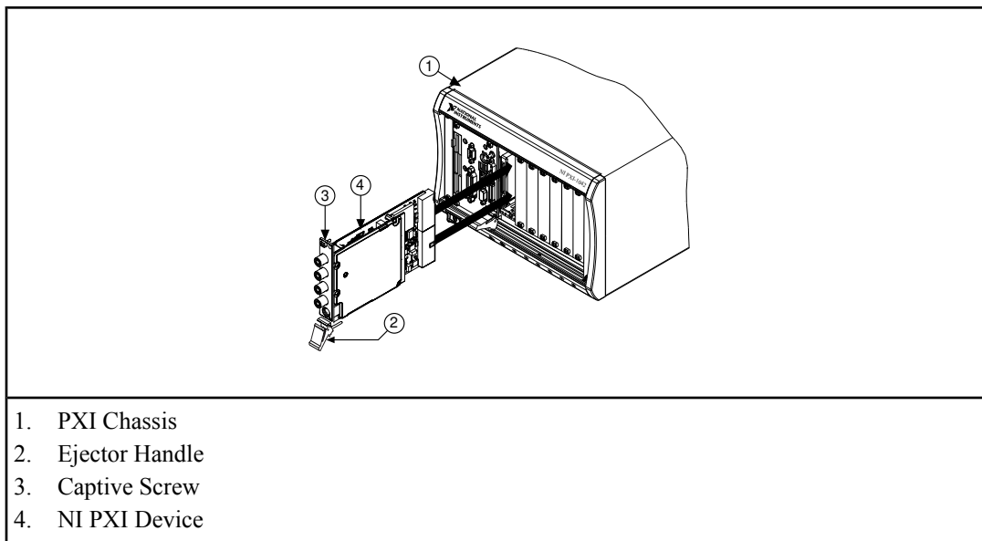
Figure 1. PXI Installation
