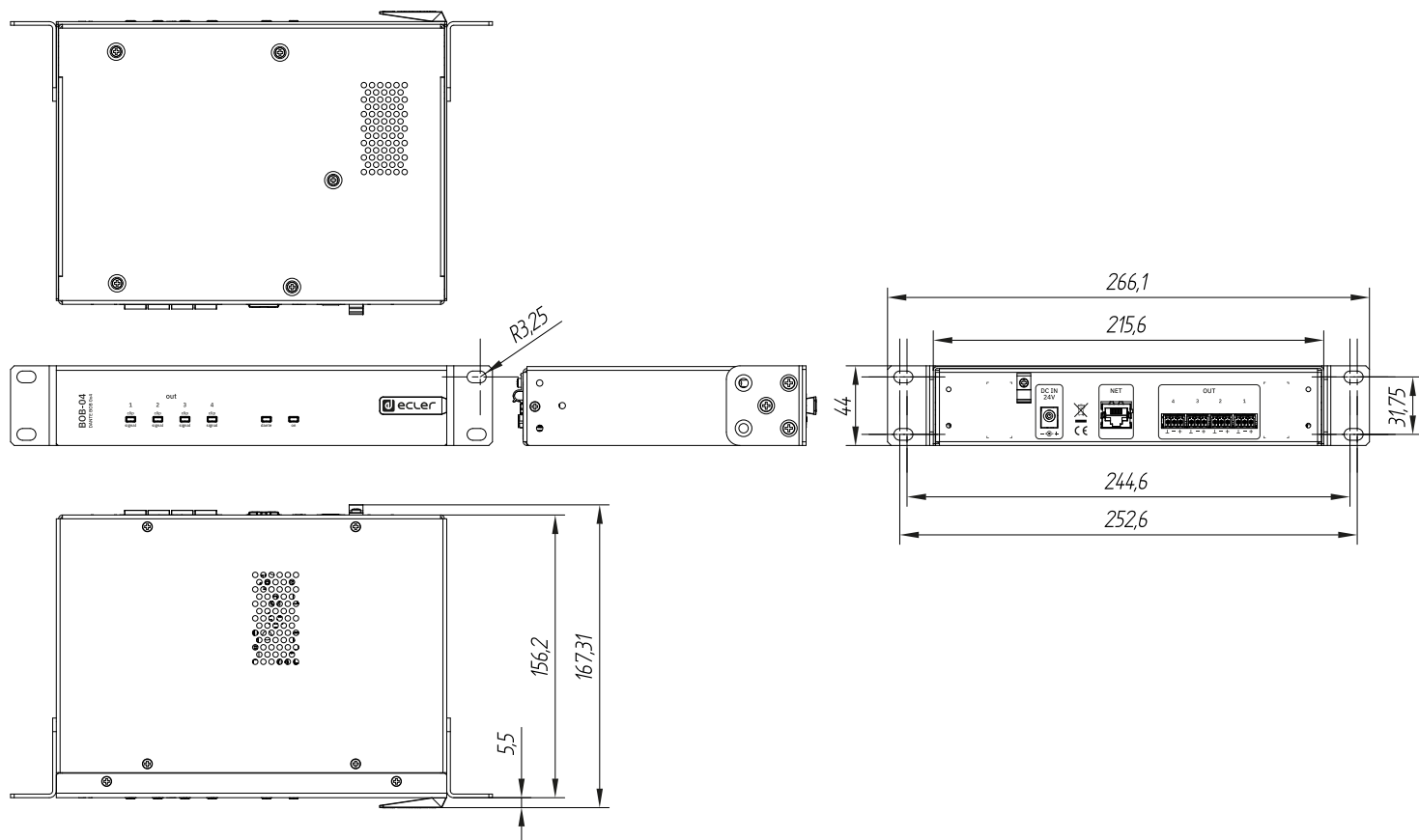
Ecler BOB-04 Mechanical Diagram
