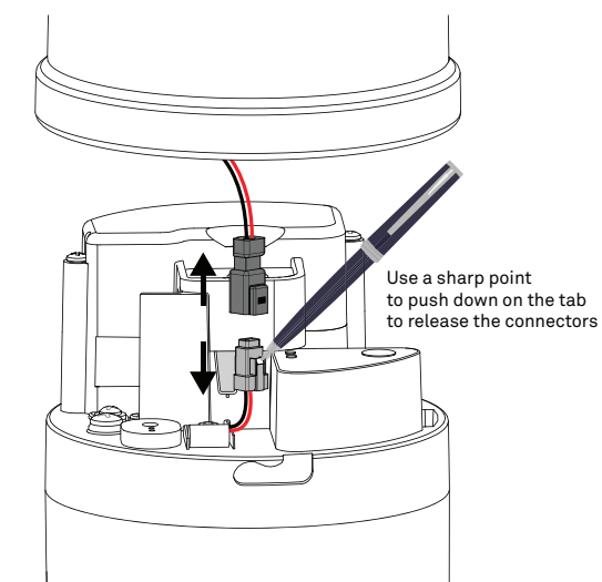
Figure 14 Disconnect pyranometer connector
