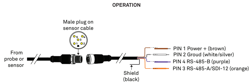
Figure 5 Four-wire M12 connector and pigtail adapter for use with screw terminals
