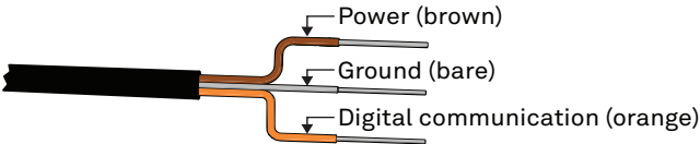
Figure 2 Pigtail wiring
