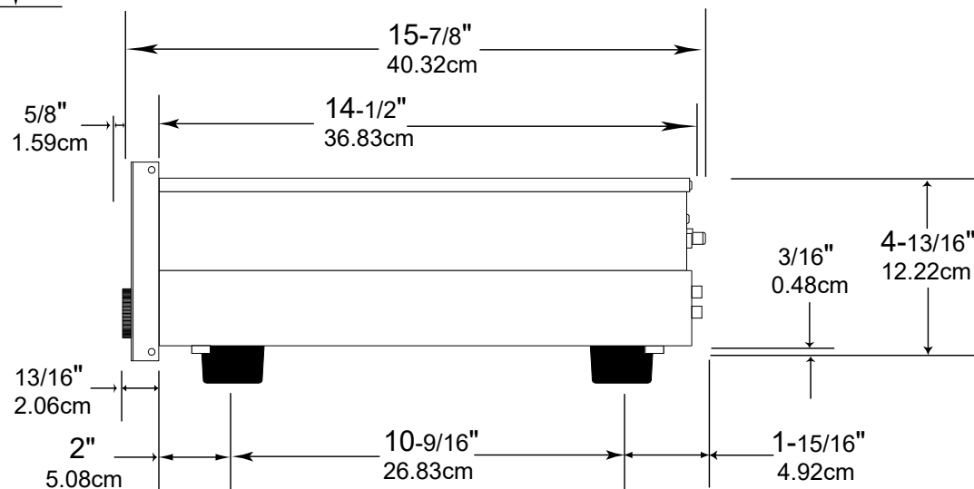
Side View of the MR89
