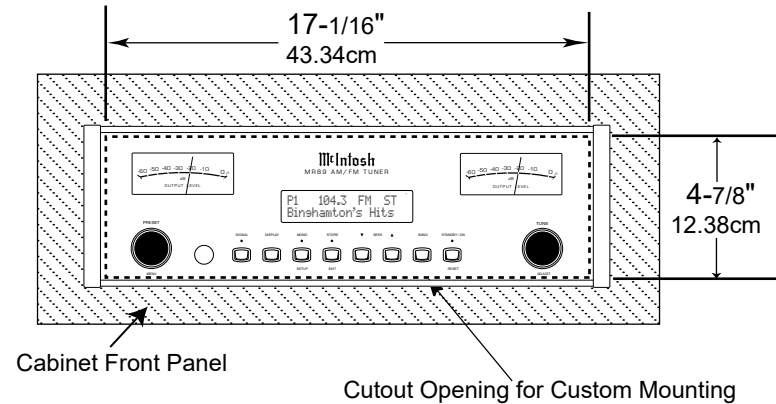
MR89 Front Panel Custom Cabinet Cutout
