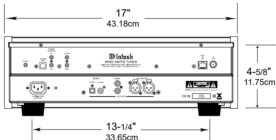
Rear View of the MR89
