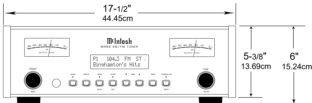
Front View of the MR89
