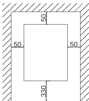
Installation clearanceview ( 1 : 10 ) (mm)
