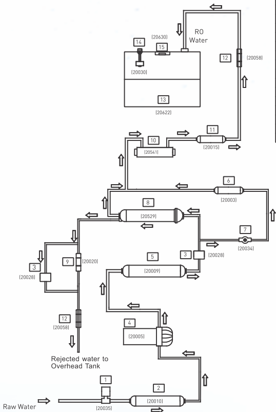
Water Flow Diagram
