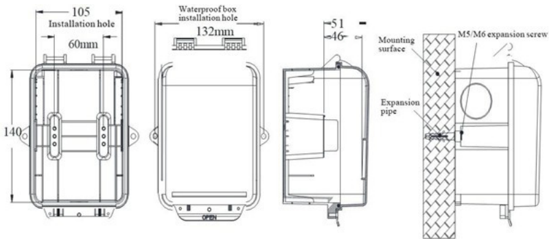
Fig.2 Installation diagram
