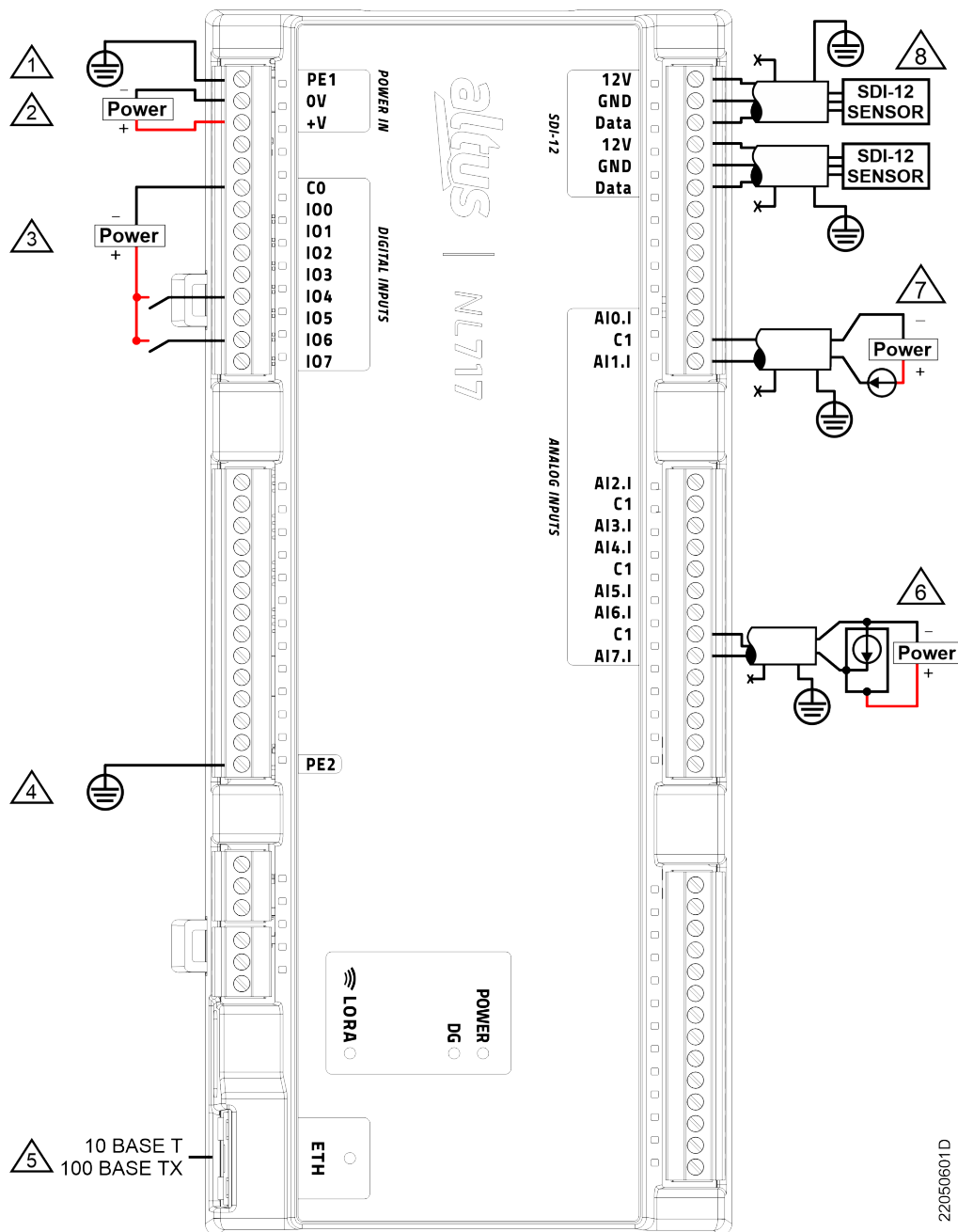
Figure 1: Electrical Installation
