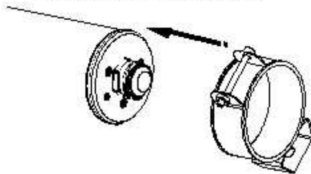
Figure 1. Attaching the Clamp Brackets (Step 3)
