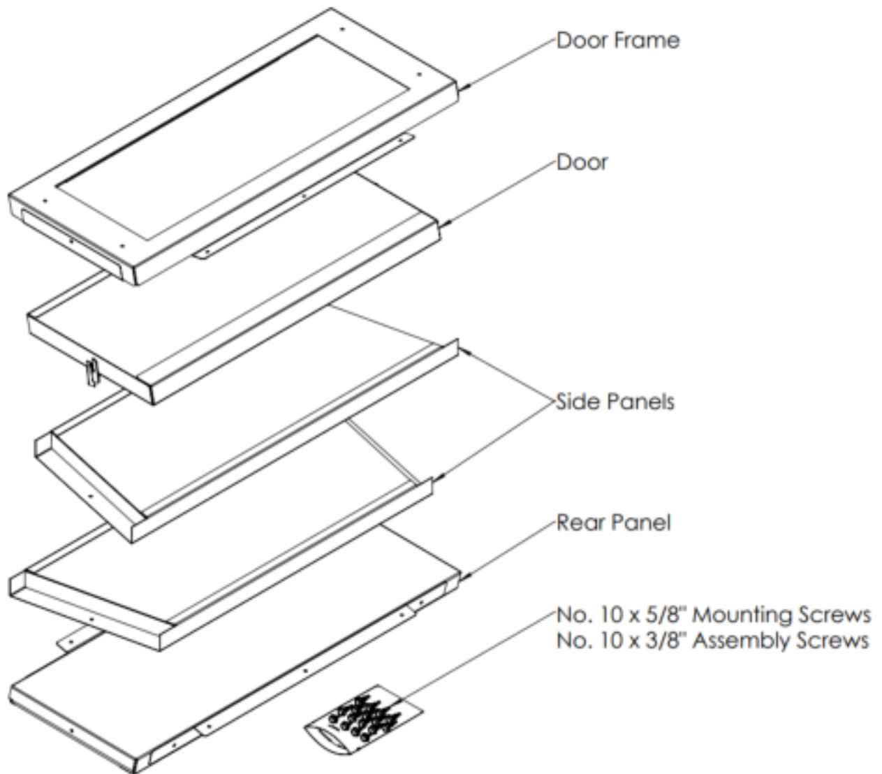
Figure 1: Components included inside the box.
