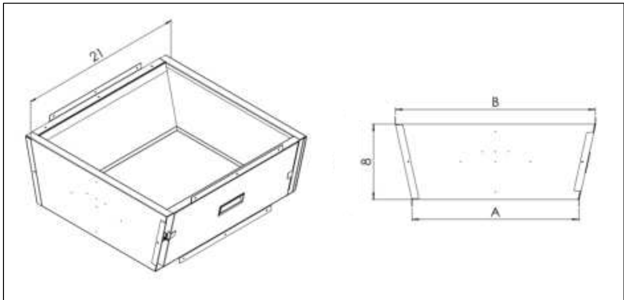
Figure 2: Unit dimensions.
