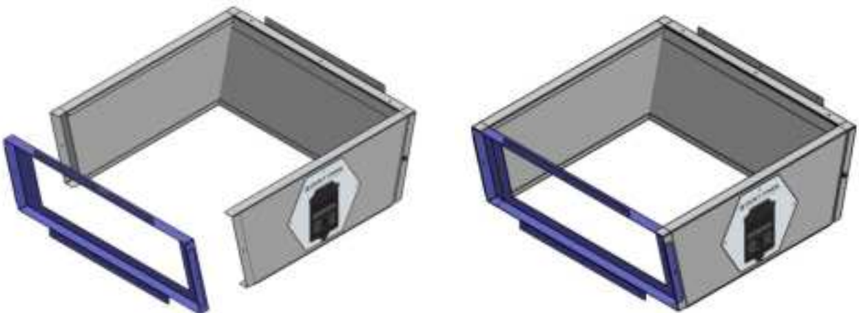
Figure 7: Door frame and unit alignment and assembly.
