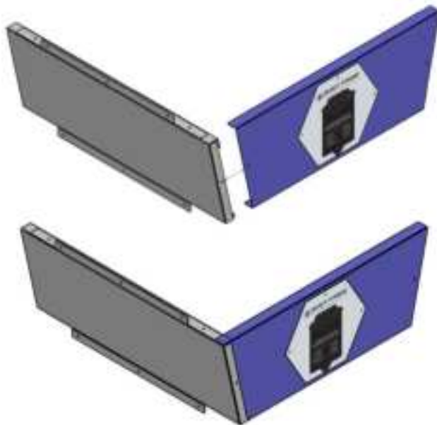
Figure 3: Side and rear panel alignment and assembly.
