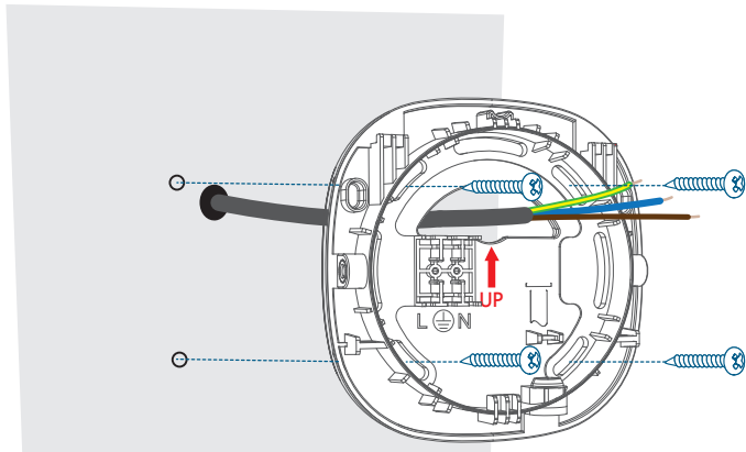
Support mural
