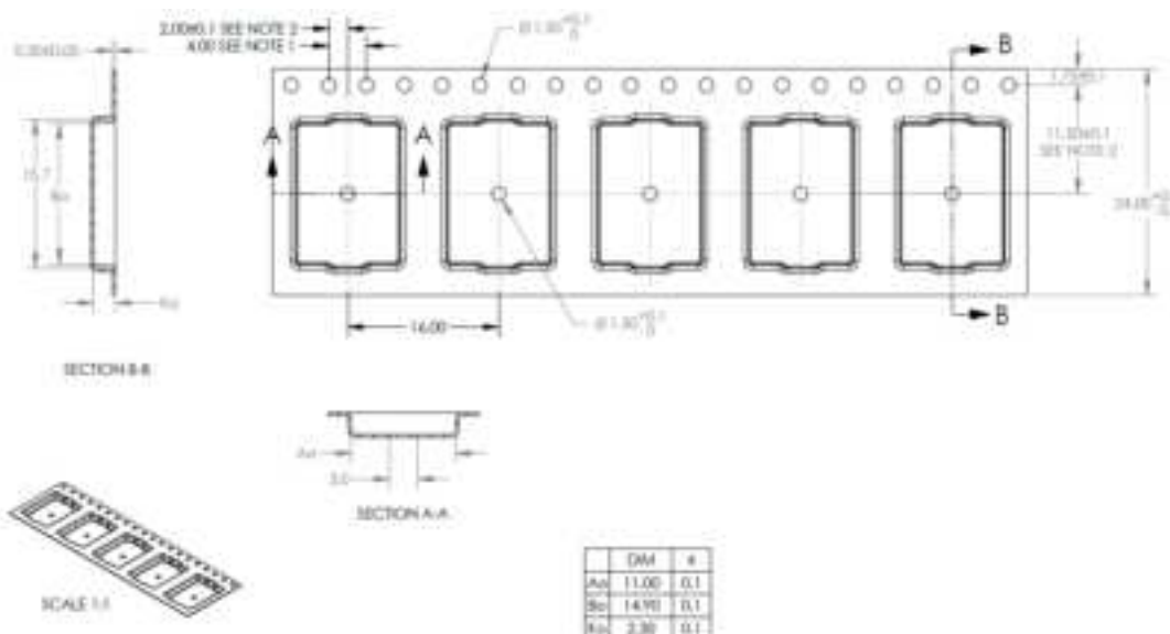
Figure 18: MAYA-W4 tape dimensions
