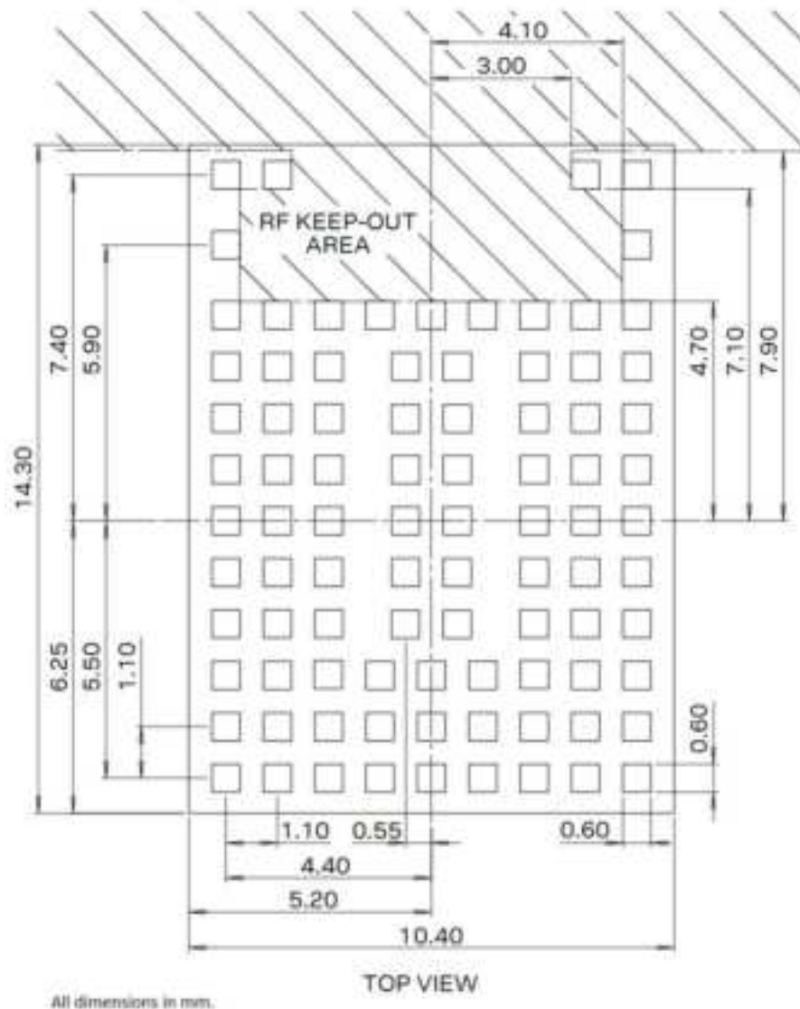
Figure 12: MAYA-W4 footprint
