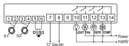
Image III - Connection 12 Vac/dc
