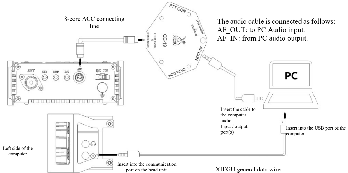
Schematic Diagram of Wiring for G90/S Data Communication using the older CE-19 box
