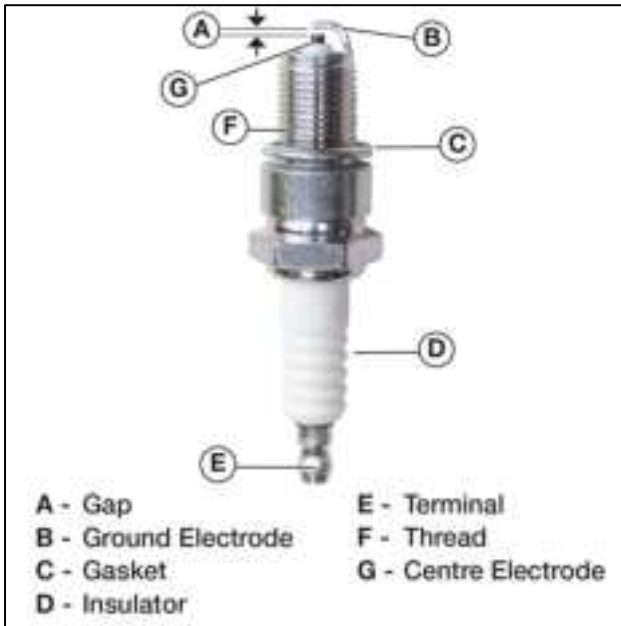
Figure 31 Spark Plug
