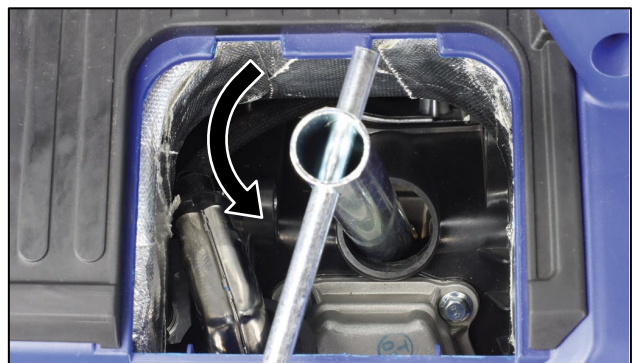
Figure 30 Remove the Spark Plug
