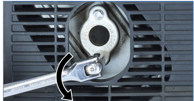
Figure 32 Remove the Spark Arrestor Clamp
