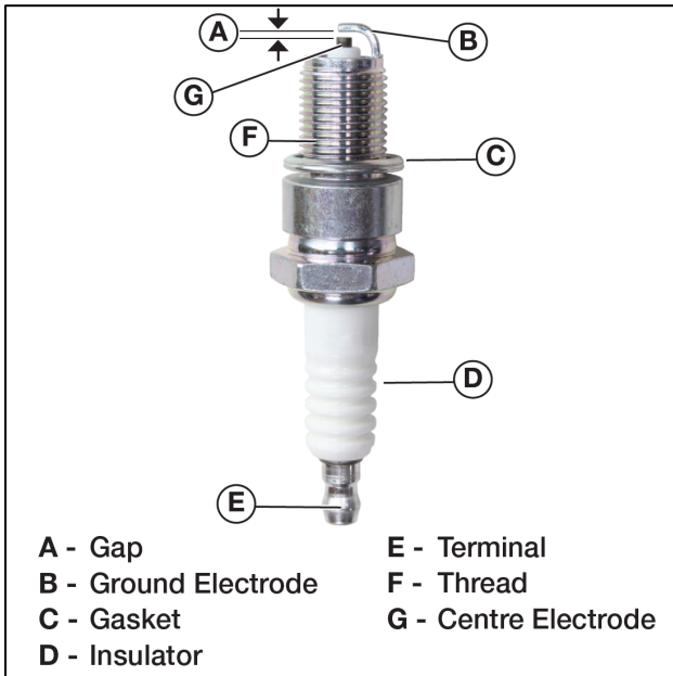
Figure 31 Spark Plug
