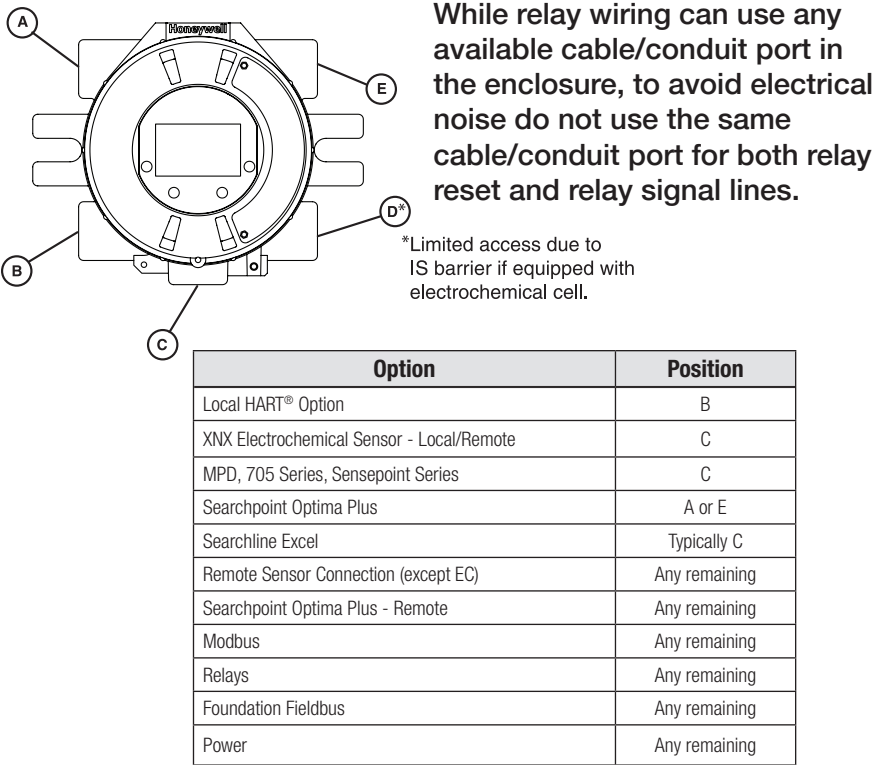
Figure 23. Cable/conduit port assignments
