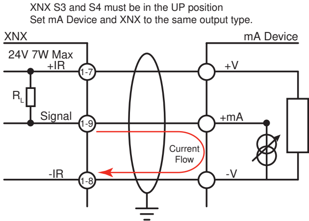
Figure 47. XNX mA input sink configuration
