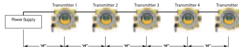
Figure 31. Daisy-chained transmitter distances
