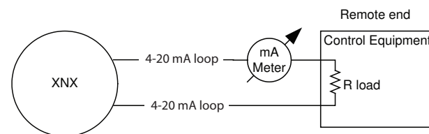
Figure 220. 4-20 mA loop with mA meter
