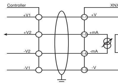
Figure 36. Isolated wiring
