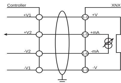
Figure 36. Isolated wiring
