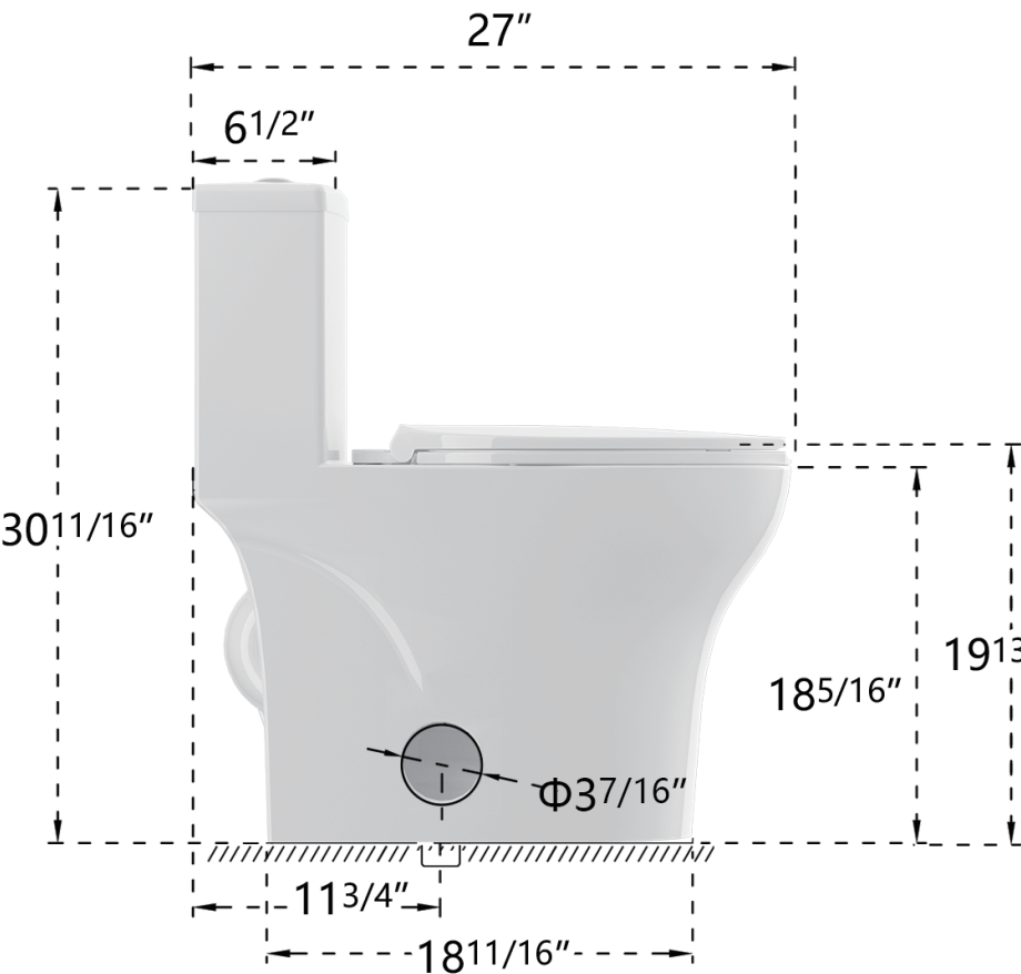
SIDE VIEW
