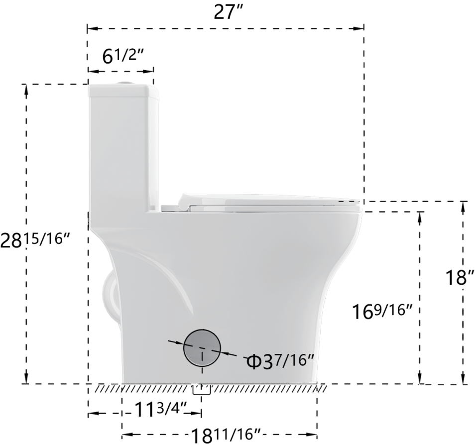
SIDE VIEW
