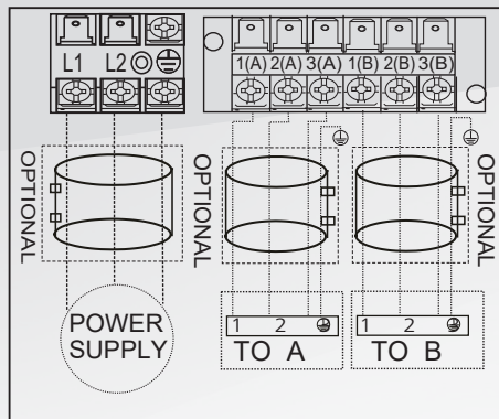
DIY-MULTI2-18HP230C (Up to 2 zones)
