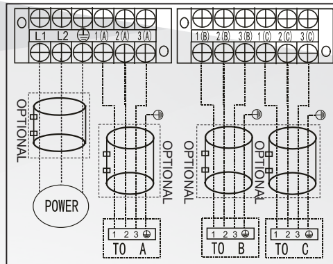
DIY-MULTI3-27HP230C (Up to 3 zones)
