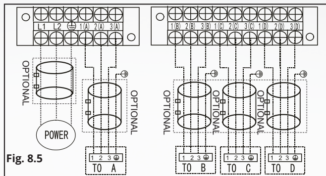
DIY-MULTI4-36HP230C (Up to 4 zones)
