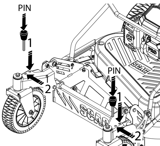
Figure 4-6. Caster Wheel Swivel / Lock
