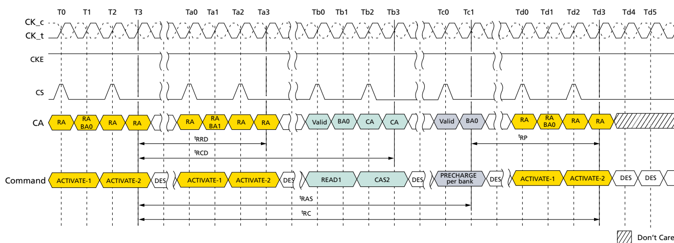
Figure 11: ACTIVATE Command
