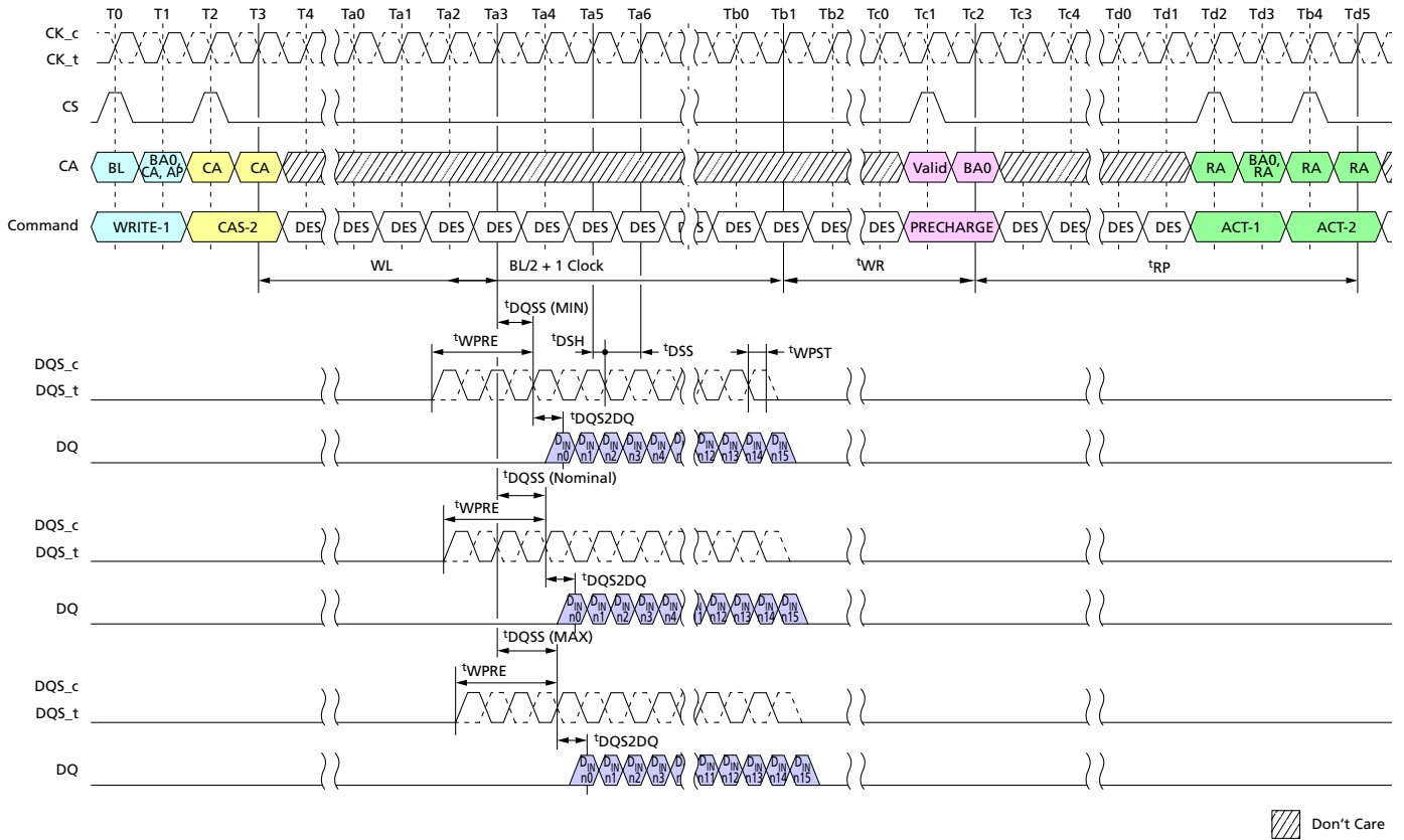
Figure 25: Burst WRITE Operation
