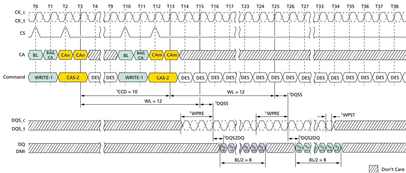
Figure 56: Consecutive WRITE: t_{CCD} = MIN + 2, 0.5nCK Postamble
