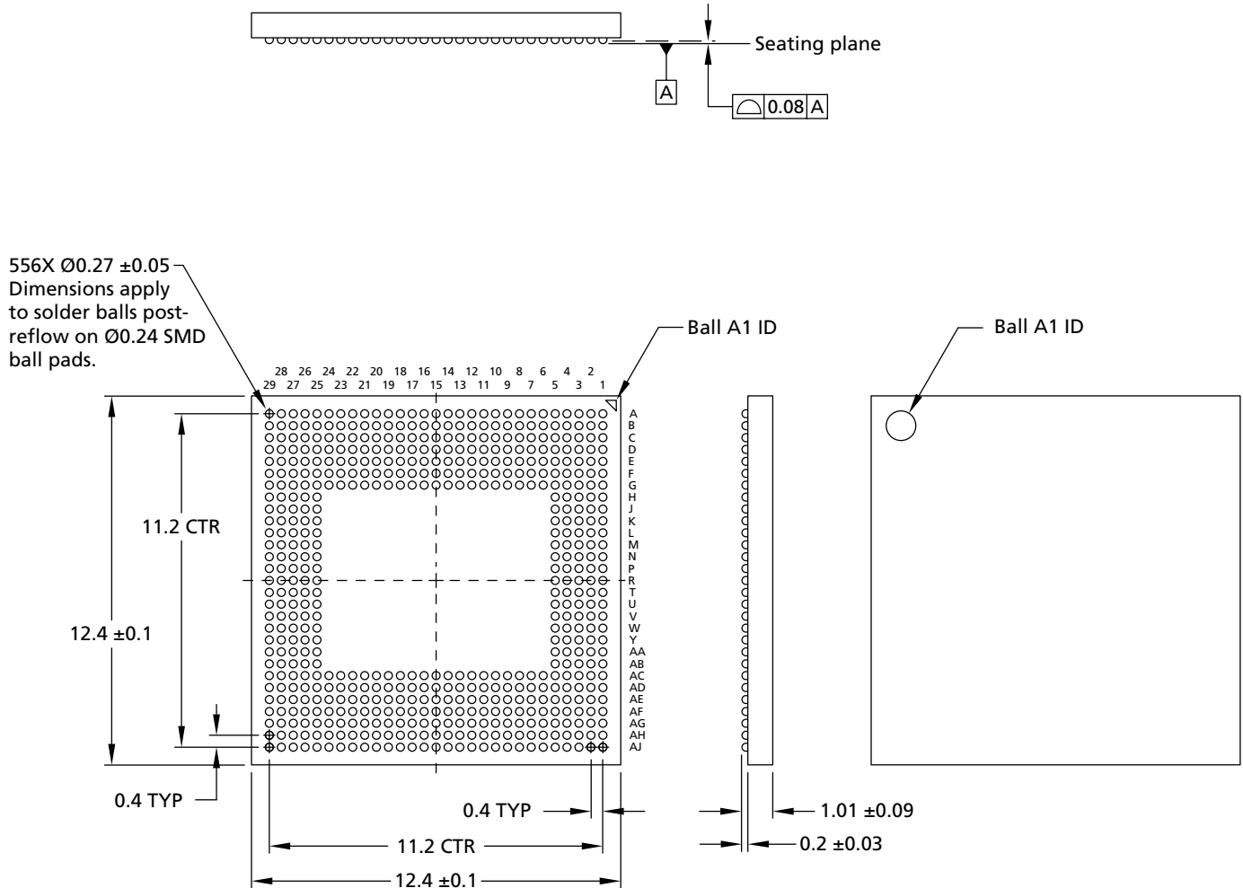
Figure 7: 556-Ball TFBGA – 12.4mm x 12.4mm x 1.1mm
