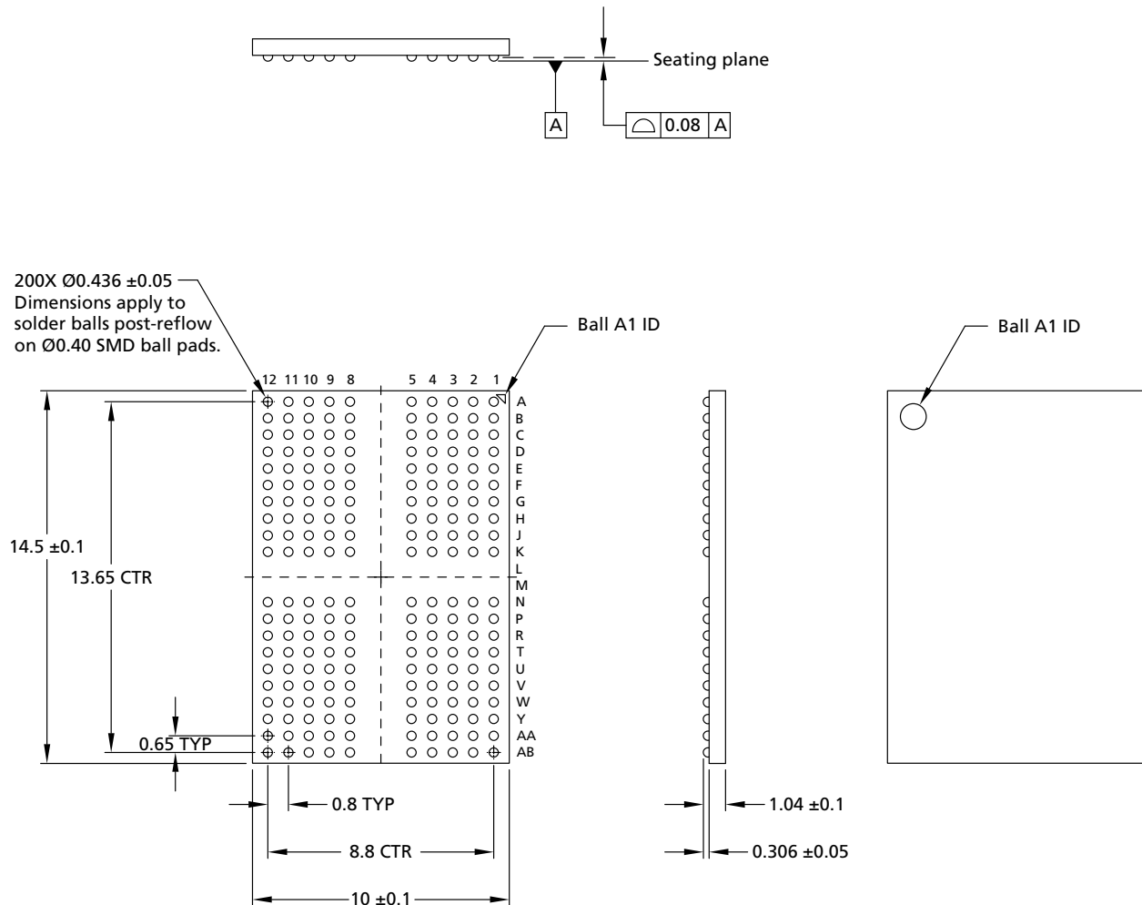
Figure 6: 200-Ball TFBGA – 10mm x 14.5mm x 1.14mm
