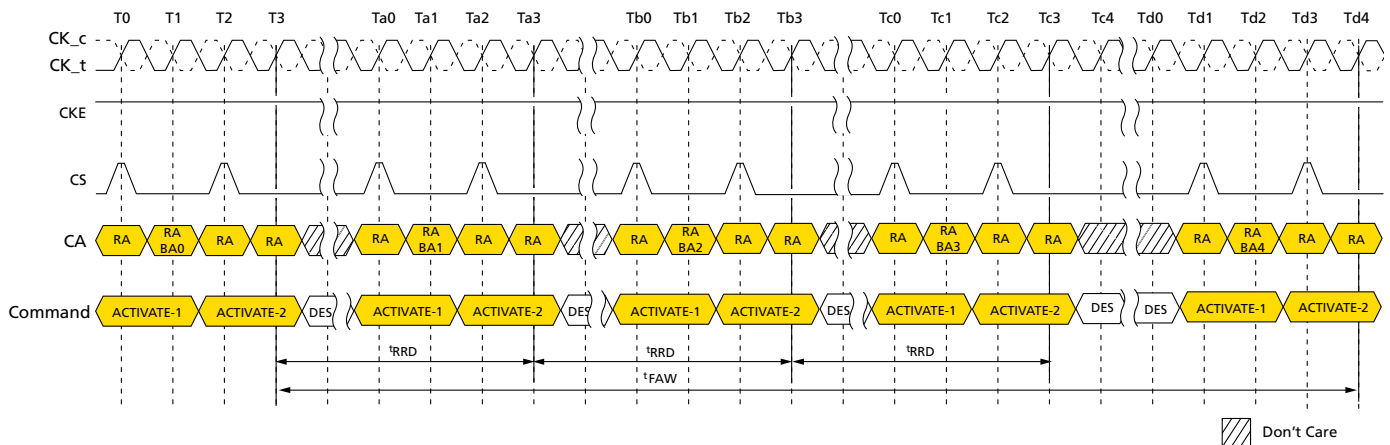
Figure 12: t_{FAW} Timing
