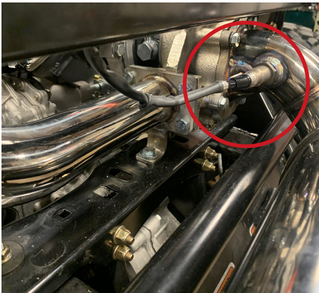
23. Install Dynojet AFR sensor into turbo exhaust. Run wires along right side of vehicle into the front cab area of the machine. Take care not to pinch or install the wire where damage can occur. Plug color matched wires into AFR Module
