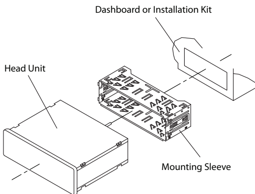
TYPICAL FRONT-LOAD DIN MOUNTING METHOD
